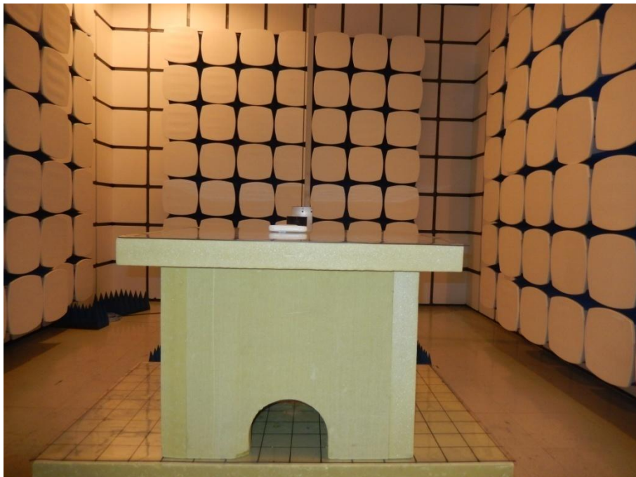
radiation H
