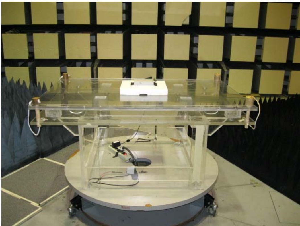
Radiated Emissions, Spurious, Front
