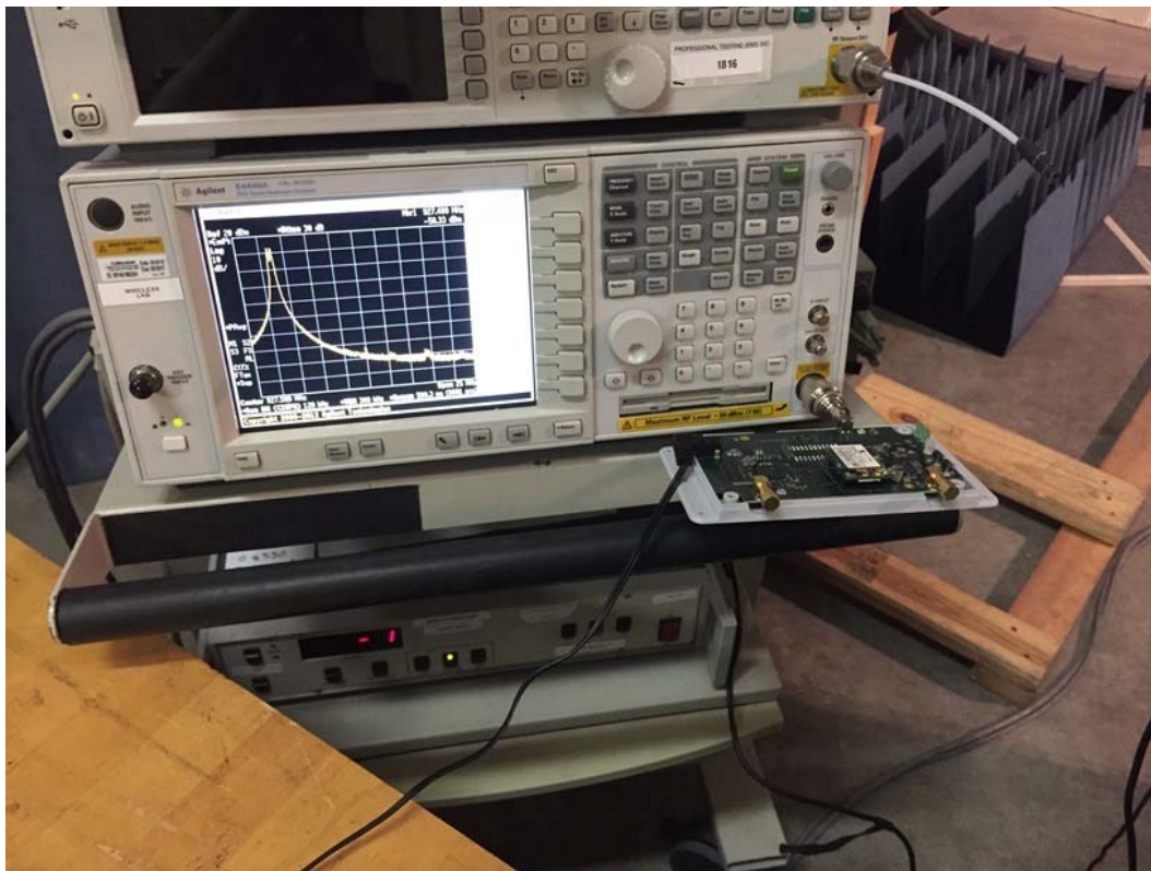
Conducted Power, BW, PSD, Bandedge, Timing, and Spurious
