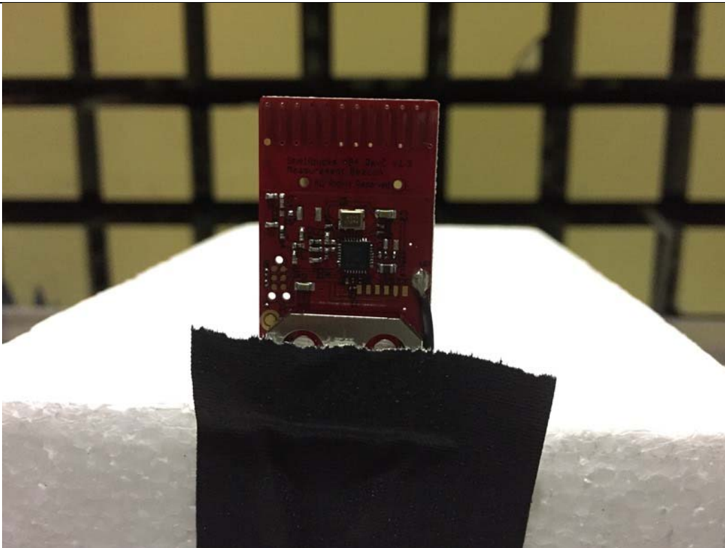
Radiated Emissions, Detail
