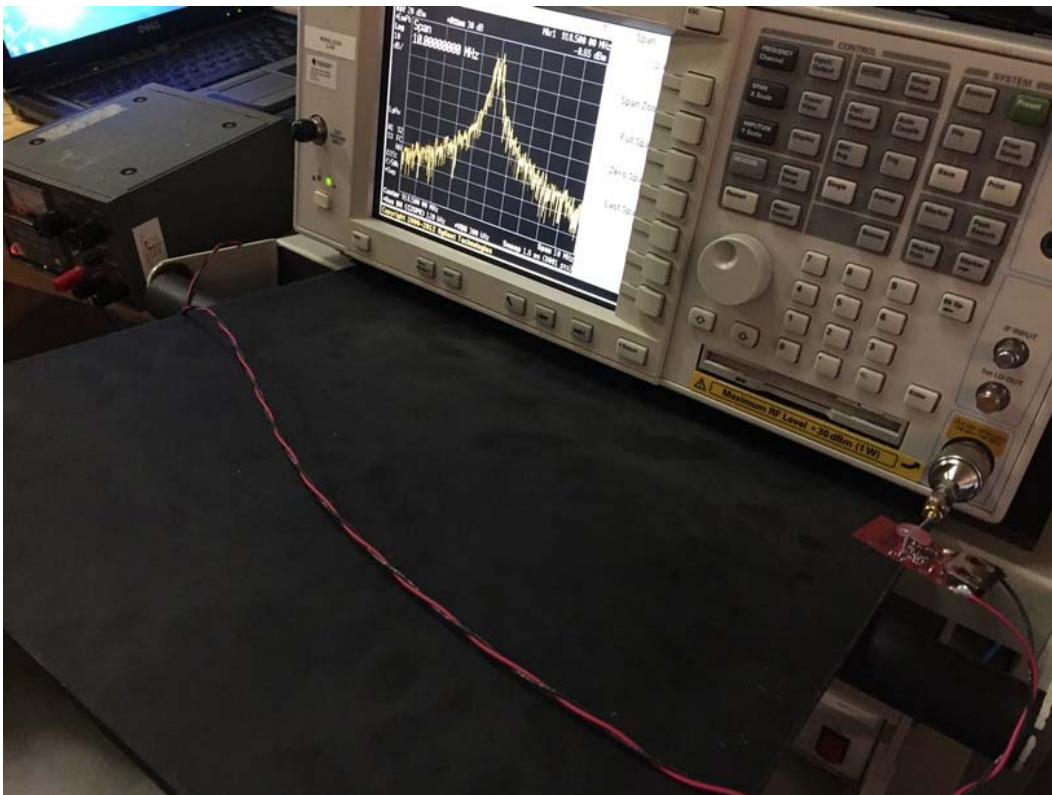
Conducted Antenna Port Measurements; Power, PSD, BW, and Band Edge
