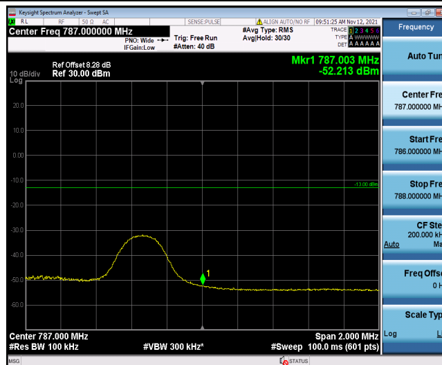
Band13-5MHz-QPSK-23255-1RB#24
