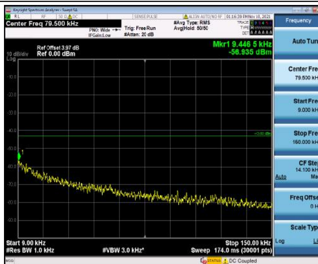
Band2-9538-4-0.009~0.15MHz
