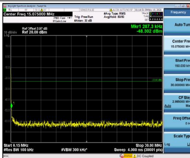
Band2-9400-4-0.15~30MHz
