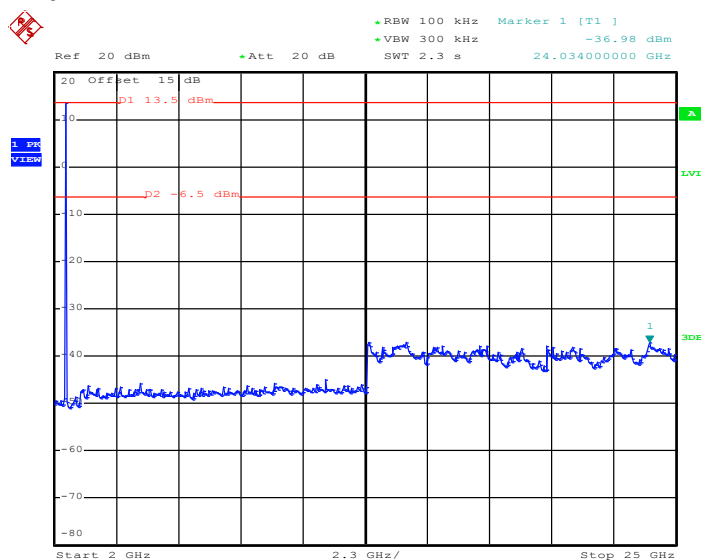
2Mbps CSE Plot on Ch 39 between 2 GHz ~ 25 GHz
