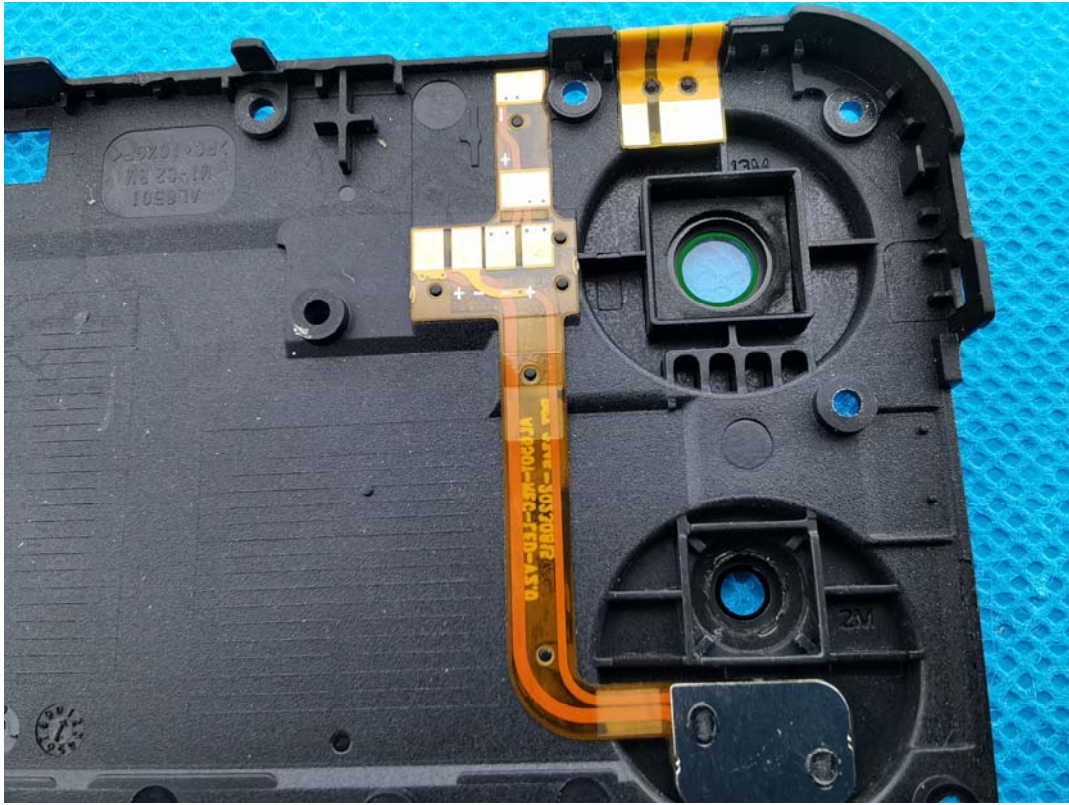
WIFI/BT/BLE/GPS Antenna
