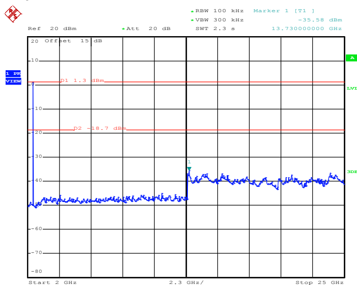
3Mbps CSE Plot on Ch 00 between 2 GHz ~ 25 GHz
