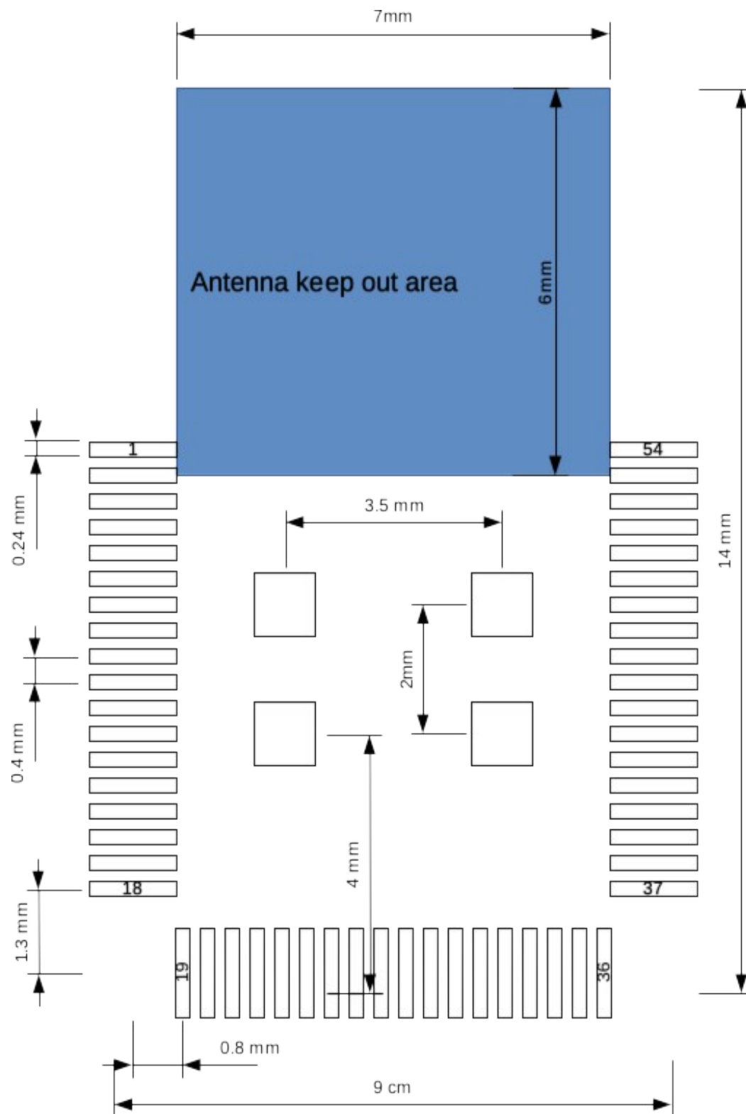
Fig. 3: SMD footprint
