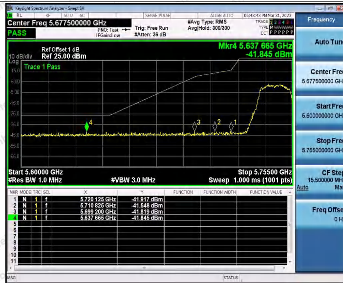
11AC20SISO_Ant2_Low_5745
