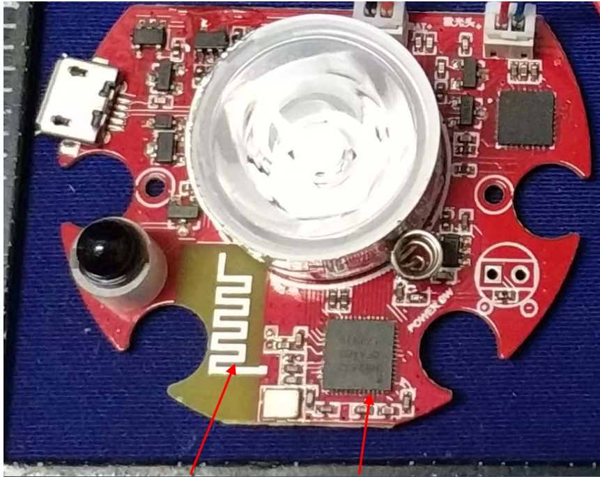
BT Antenna
