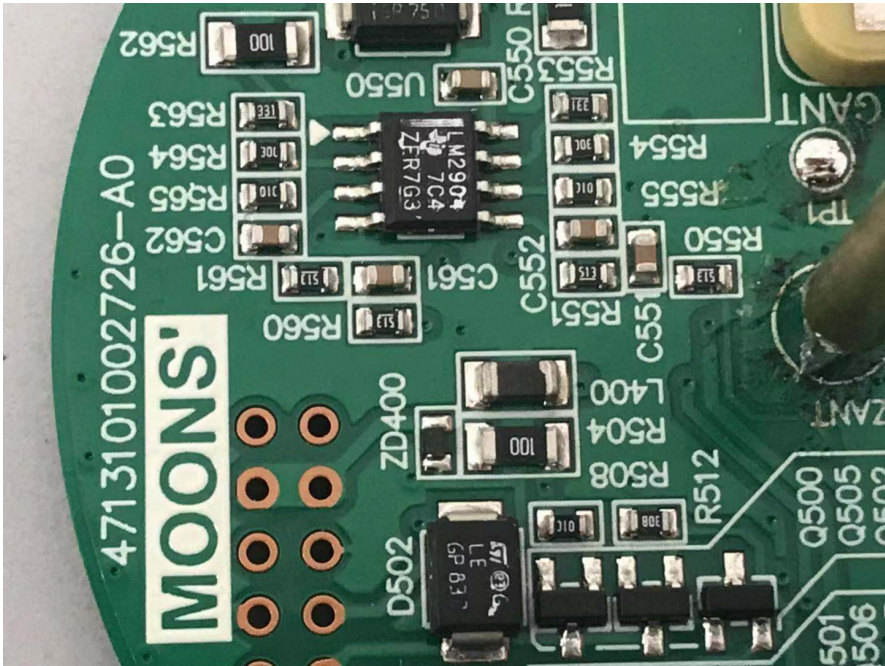
EUT – PCB-1 Top Chip View-3
