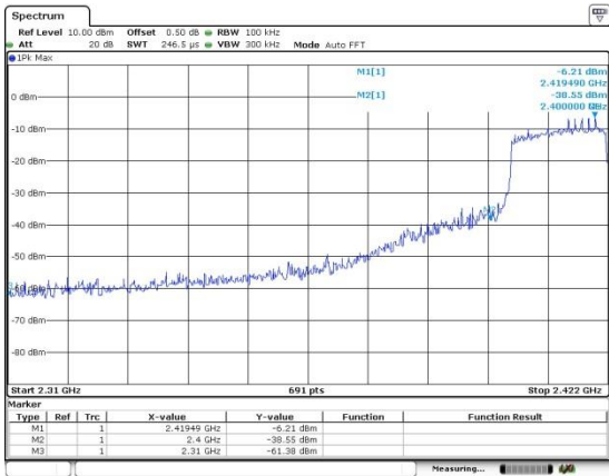
CH03-Bandedge
