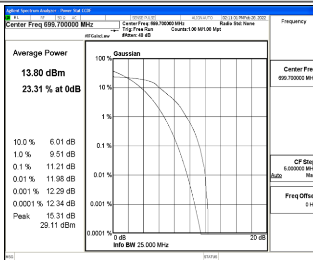
Band12-1.4MHz-16QAM-23017-6-0-Low-11.21-<=13-PASS
