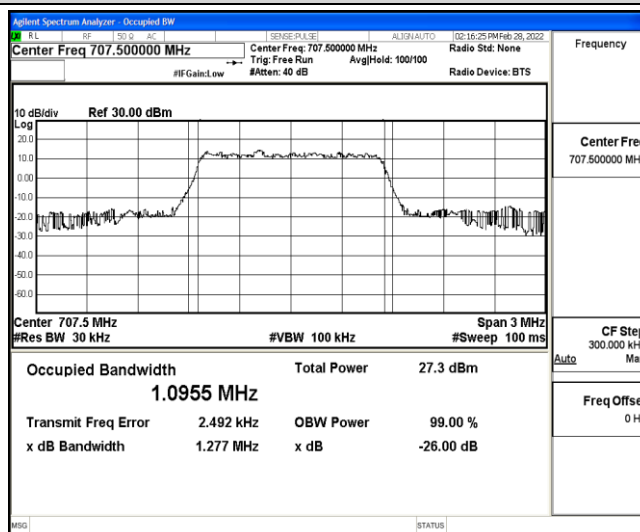
Band12-1.4MHz-16QAM-23095-6-0-Low-1.0955-1.277-PASS
