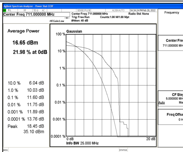
Band12-10MHz-16QAM-23130-1-0-High-11.60-13-PASS
