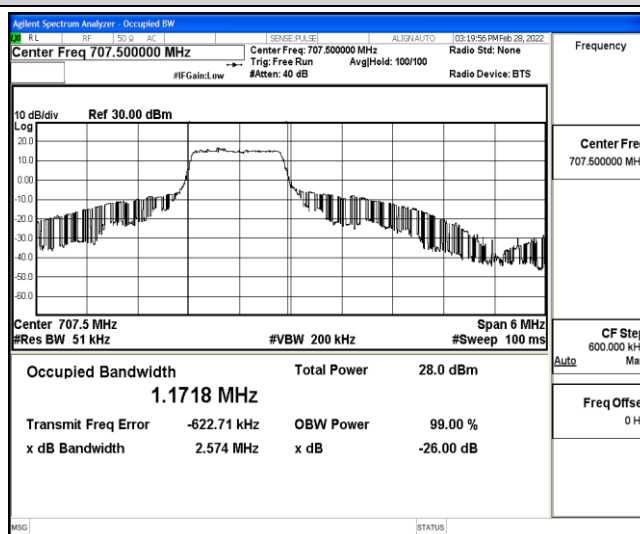
Band12-3MHz-QPSK-23095-6-0-Low-1.1718-2.574-PASS
