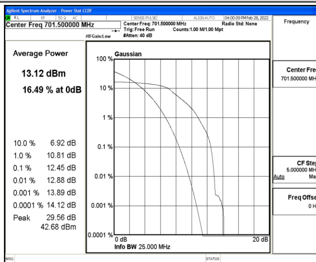
Band12-5MHz-16QAM-23035-6-0-Low-12.45-<=13-PASS
