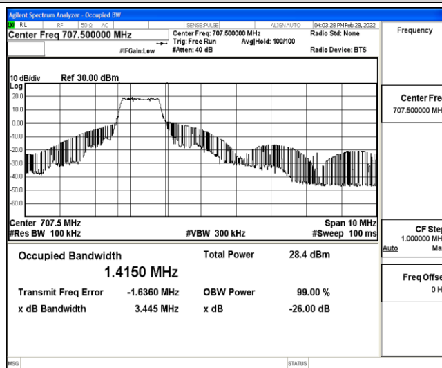
Band12-5MHz-QPSK-23095-6-0-Low-1.4150-3.445-PASS
