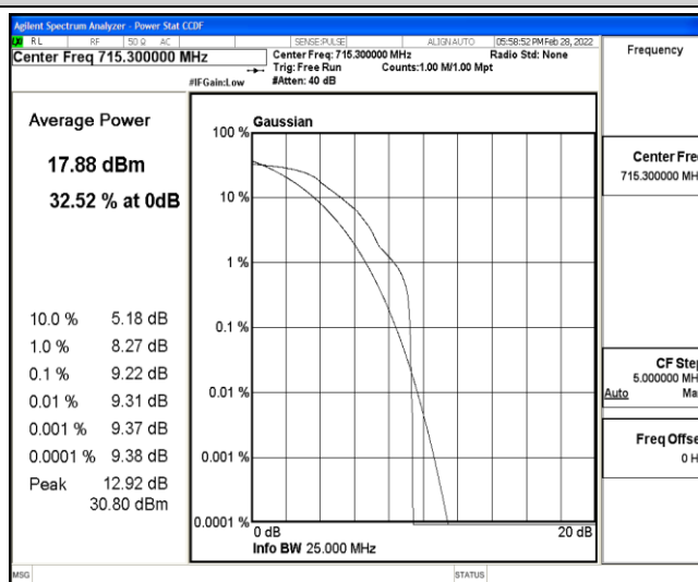
Band12-1.4MHz-QPSK-23173-1-0-High-9.22-<=13-PASS
