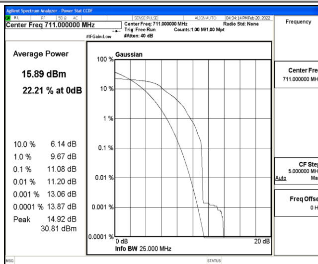
Band12-10MHz-QPSK-23130-1-0-High-11.08-<=13-PASS
