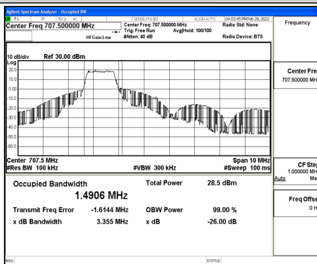
Band12-5MHz-16QAM-23095-6-0-Low-1.4906-3.355-PASS
