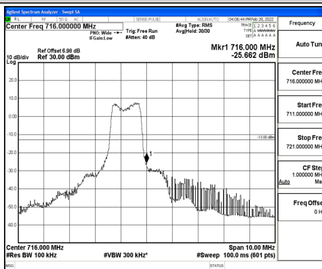
Band12-5MHz-16QAM-23155-6-0-High--25.66-PASS
