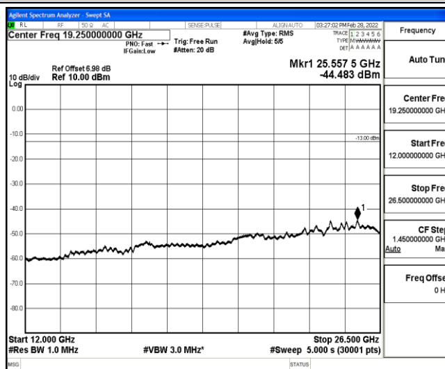
Band12-3MHz-QPSK-23025-1-0-Low-12000-26500--44.48-PASS
