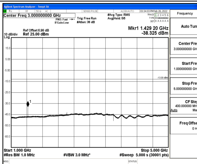
Band12-3MHz-QPSK-23165-1-0-High-1000-5000--38.33-PASS
