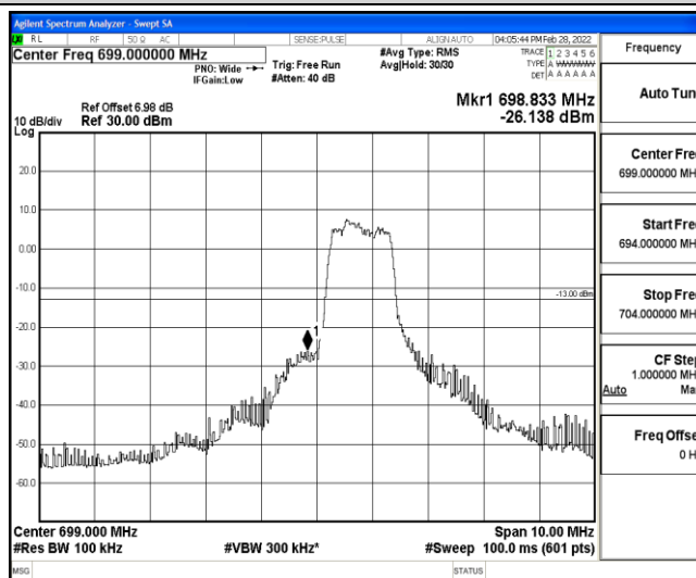
Band12-5MHz-QPSK-23035-6-0-Low--26.14-PASS
