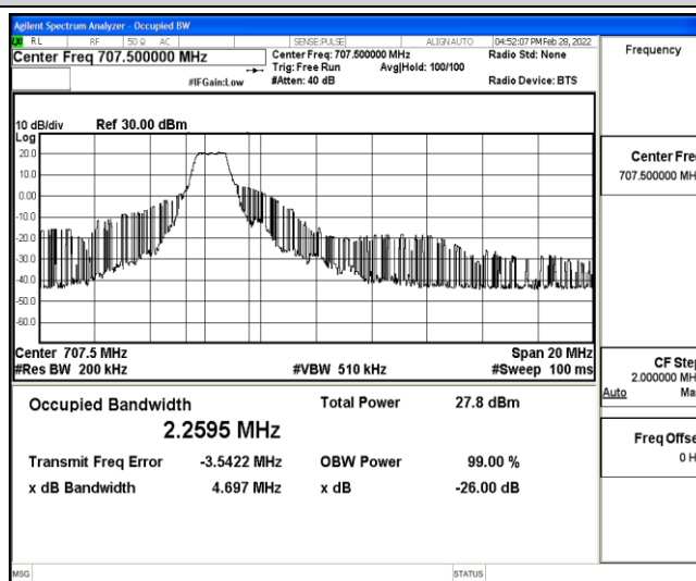
Band12-10MHz-16QAM-23095-6-0-Low-2.2595-4.697-PASS
