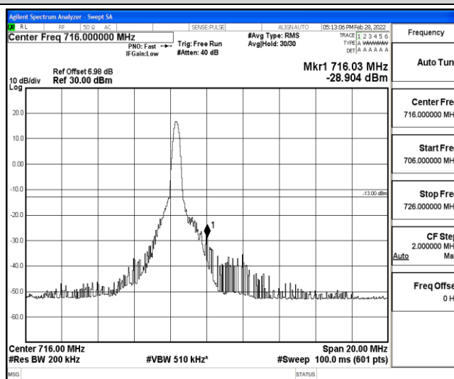
Band12-10MHz-QPSK-23130-1-0-High--28.90-PASS
