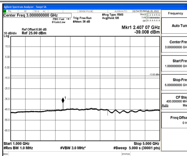
Band12-1.4MHz-QPSK-23173-1-0-High-1000-5000--39.01-PASS
