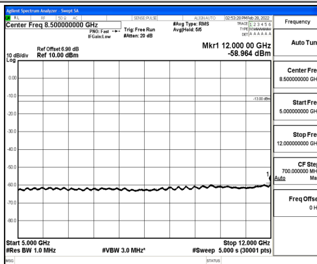
Band12-1.4MHz-16QAM-23095-1-0-Low-5000-12000--58.96-PASS
