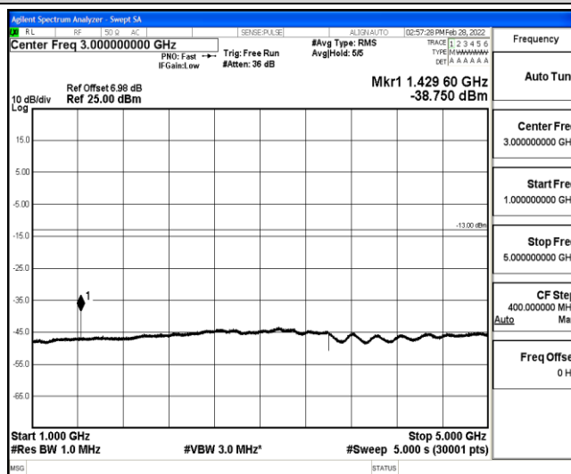
Band12-1.4MHz-16QAM-23173-1-0-High-1000-5000--38.75-PASS
