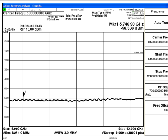
Band12-3MHz-QPSK-23095-1-0-Low-5000-12000--58.37-PASS
