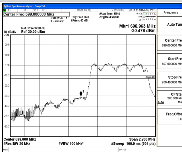
Band12-1.4MHz-16QAM-23017-6-0-Low--30.48-PASS
