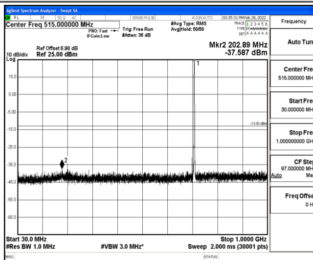
Band12-3MHz-16QAM-23165-1-0-High-30-1000--37.59-PASS
