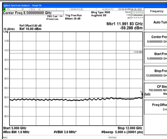
Band12-3MHz-16QAM-23165-1-0-High-5000-12000--59.29-PASS
