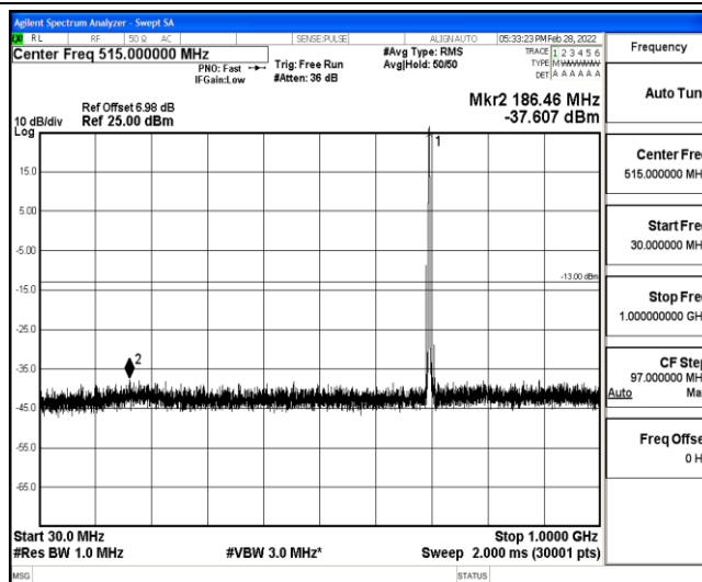
Band12-10MHz-16QAM-23095-1-0-Low-30-1000--37.61-PASS
