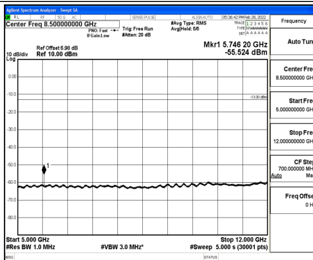
Band12-10MHz-QPSK-23130-1-0-High-5000-12000--55.52-PASS
