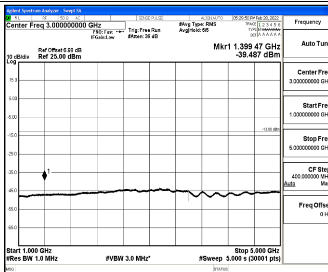
Band12-10MHz-16QAM-23060-1-0-Low-1000-5000--39.49-PASS
