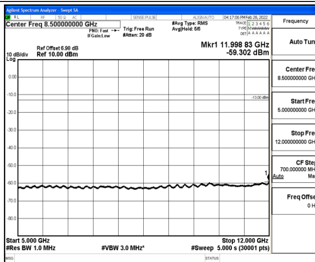
Band12-5MHz-QPSK-23155-1-0-High-5000-12000--59.3-PASS
