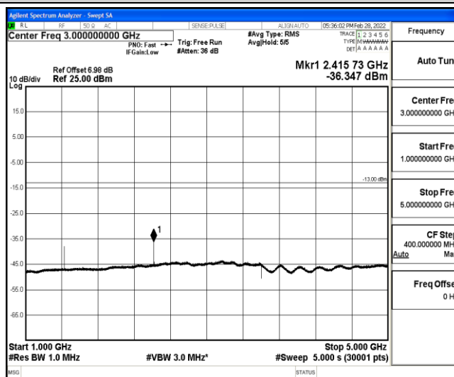
Band12-10MHz-QPSK-23130-1-0-High-1000-5000--36.35-PASS
