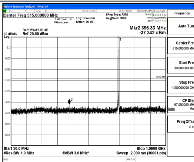
Band12-10MHz-16QAM-23060-1-0-Low-30-1000--37.34-PASS
