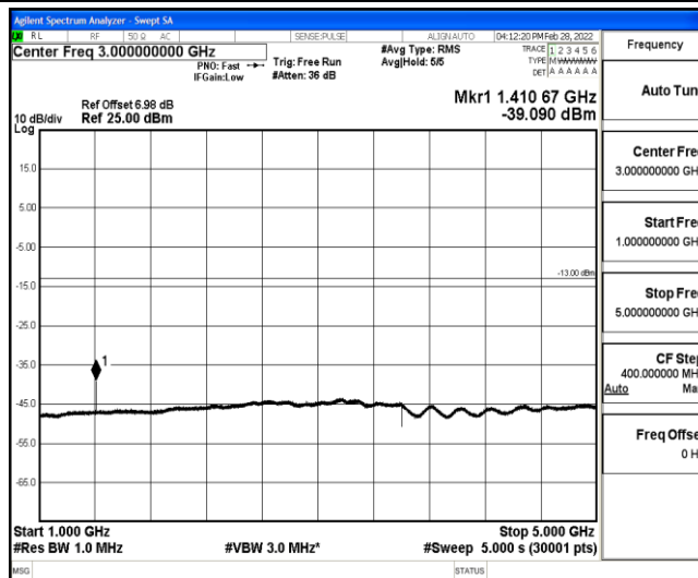
Band12-5MHz-QPSK-23095-1-0-Low-1000-5000--39.09-PASS
