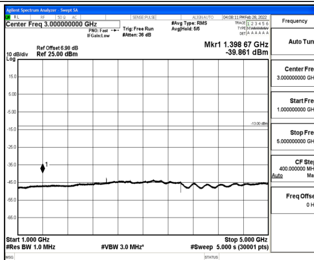
Band12-5MHz-QPSK-23035-1-0-Low-1000-5000--39.86-PASS
