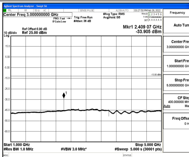
Band12-3MHz-16QAM-23025-1-0-Low-1000-5000--33.91-PASS
