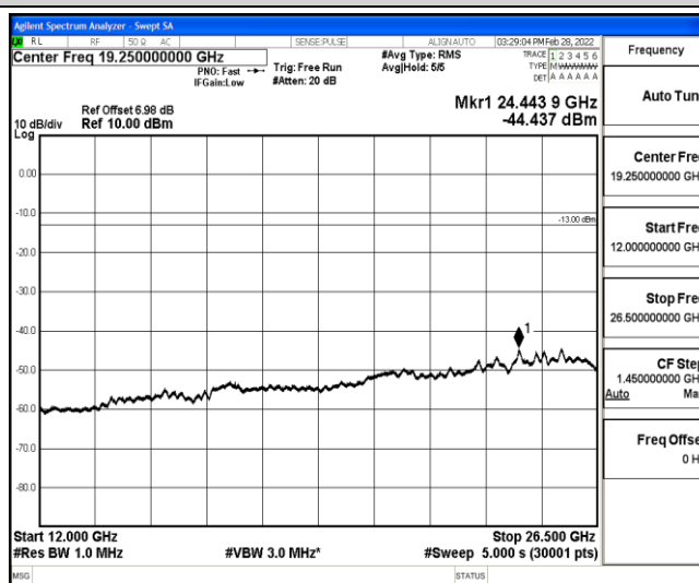
Band12-3MHz-16QAM-23025-1-0-Low-12000-26500--44.44-PASS
