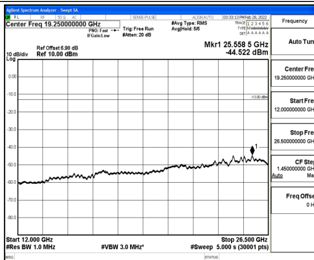
Band12-3MHz-16QAM-23095-1-0-Low-12000-26500--44.52-PASS
