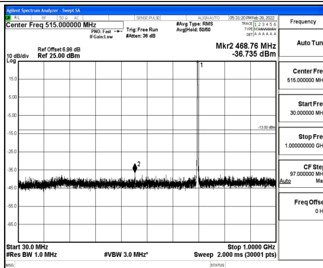
Band12-10MHz-QPSK-23095-1-0-Low-30-1000--36.74-PASS
