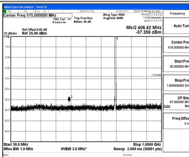
Band12-3MHz-16QAM-23025-1-0-Low-30-1000--37.36-PASS
