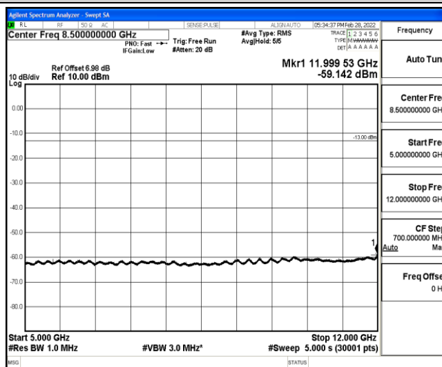
Band12-10MHz-16QAM-23095-1-0-Low-5000-12000--59.14-PASS
