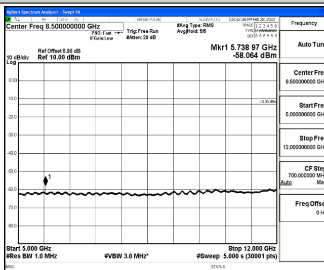
Band12-3MHz-16QAM-23095-1-0-Low-5000-12000--58.06-PASS
