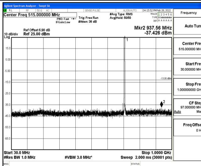
Band12-5MHz-QPSK-23155-1-0-High-30-1000--37.43-PASS
