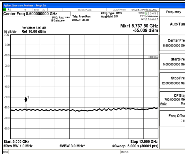
Band12-5MHz-QPSK-23035-1-0-Low-5000-12000--55.04-PASS
