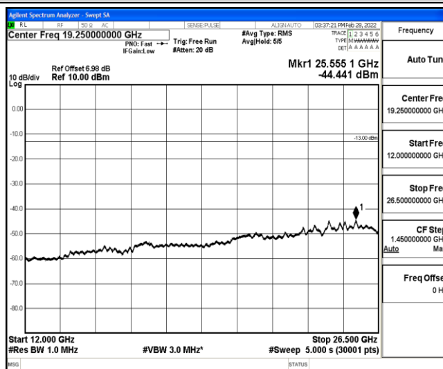
Band12-3MHz-16QAM-23165-1-0-High-12000-26500--44.44-PASS
