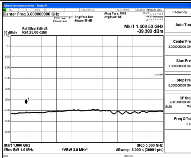
Band12-10MHz-16QAM-23095-1-0-Low-1000-5000--39.38-PASS
