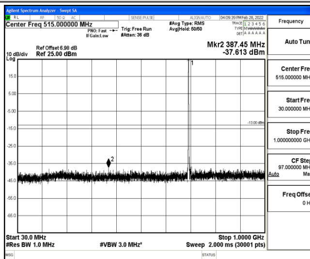
Band12-5MHz-16QAM-23035-1-0-Low-30-1000--37.61-PASS
