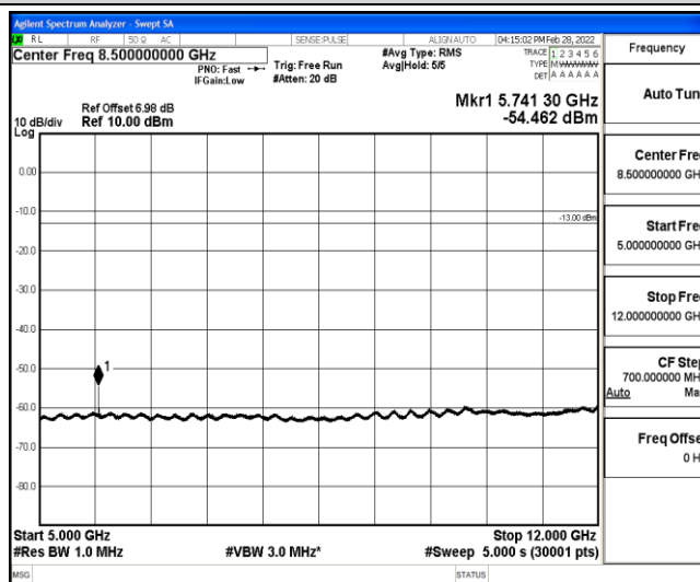
Band12-5MHz-16QAM-23095-1-0-Low-5000-12000--54.46-PASS
