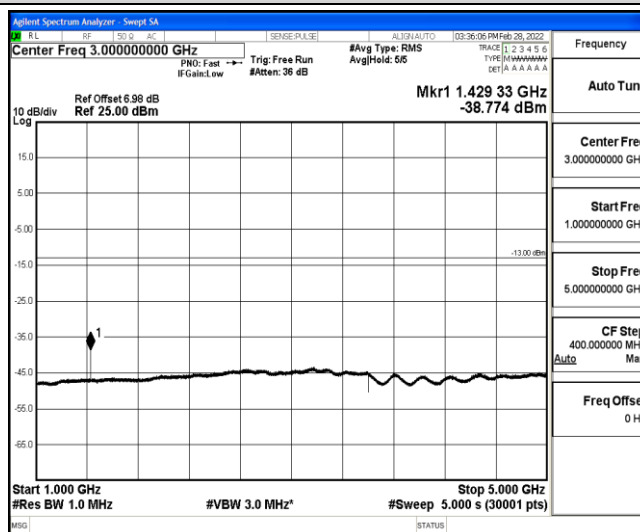
Band12-3MHz-16QAM-23165-1-0-High-1000-5000--38.77-PASS
