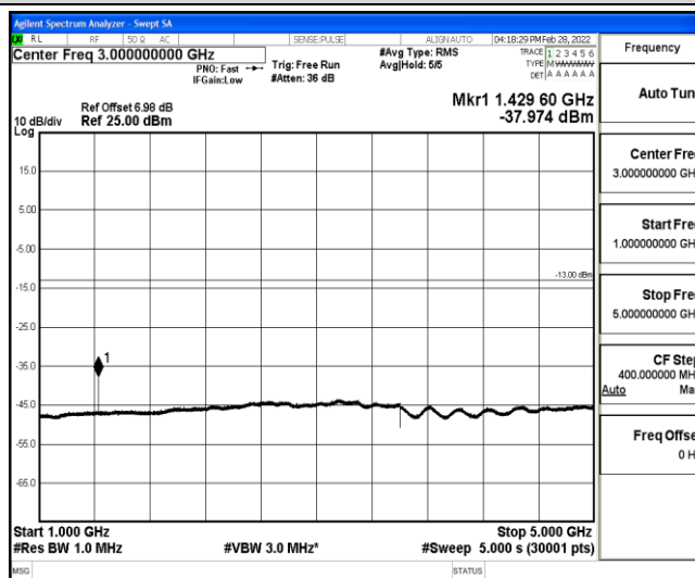
Band12-5MHz-16QAM-23155-1-0-High-1000-5000--37.97-PASS
