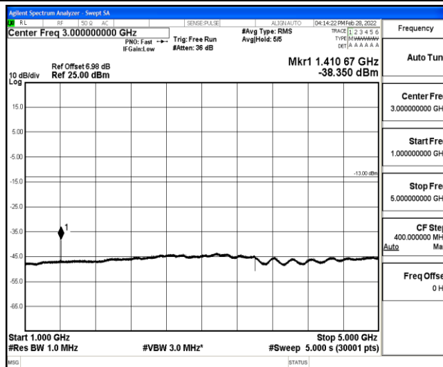
Band12-5MHz-16QAM-23095-1-0-Low-1000-5000--38.35-PASS
