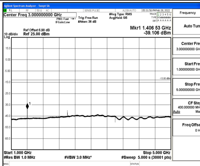
Band12-10MHz-QPSK-23095-1-0-Low-1000-5000--39.11-PASS
