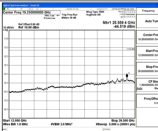
Band12-5MHz-QPSK-23035-1-0-Low-12000-26500--44.52-PASS
