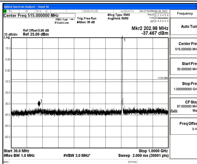
Band12-5MHz-16QAM-23155-1-0-High-30-1000--37.47-PASS
