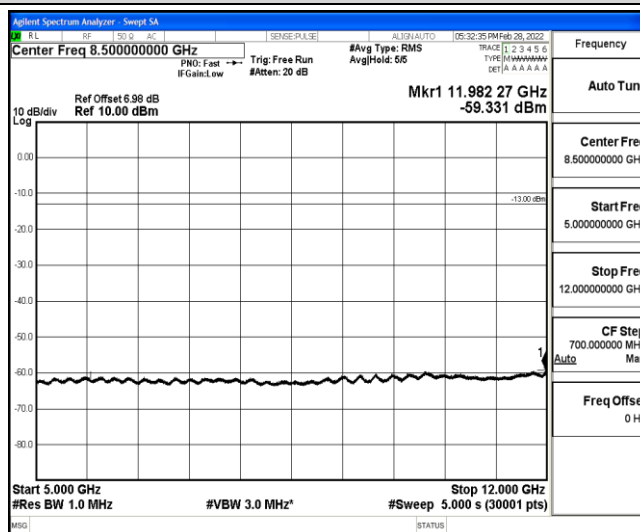
Band12-10MHz-QPSK-23095-1-0-Low-5000-12000--59.33-PASS
