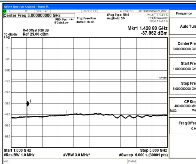
Band12-10MHz-16QAM-23130-1-0-High-1000-5000--37.85-PASS
