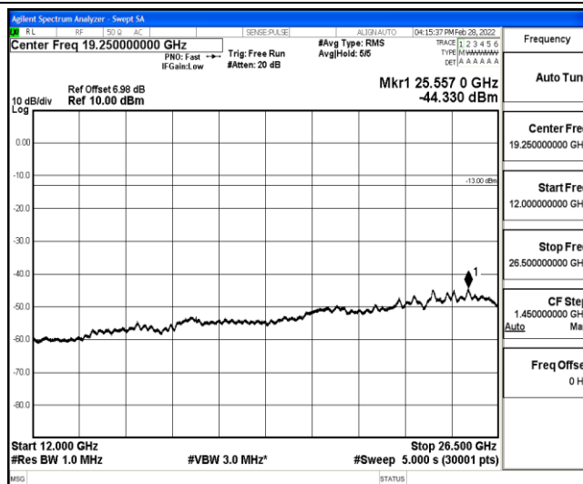
Band12-5MHz-16QAM-23095-1-0-Low-12000-26500--44.33-PASS
