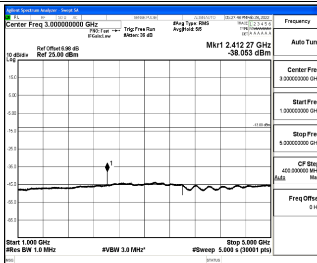
Band12-10MHz-QPSK-23060-1-0-Low-1000-5000--38.05-PASS
