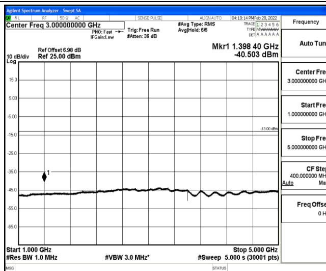
Band12-5MHz-16QAM-23035-1-0-Low-1000-5000--40.5-PASS
