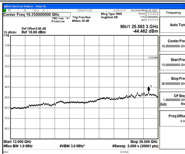
Band12-5MHz-16QAM-23155-1-0-High-12000-26500--44.46-PASS
