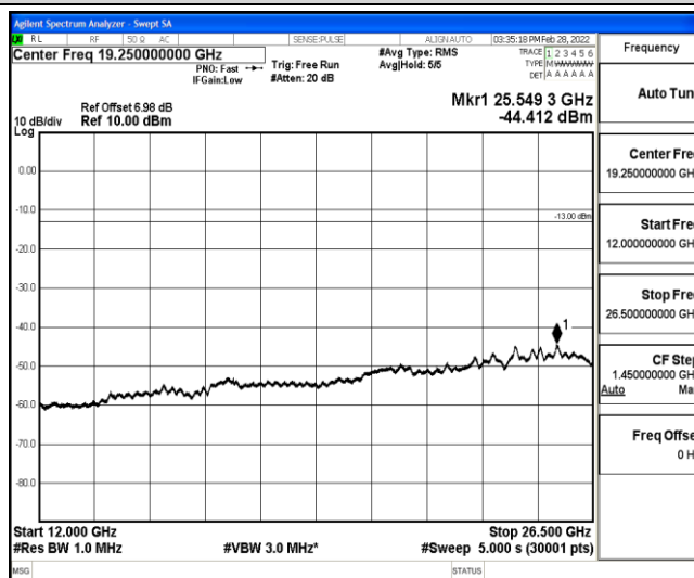
Band12-3MHz-QPSK-23165-1-0-High-12000-26500--44.41-PASS
