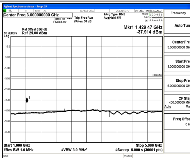
Band12-5MHz-QPSK-23155-1-0-High-1000-5000--37.91-PASS
