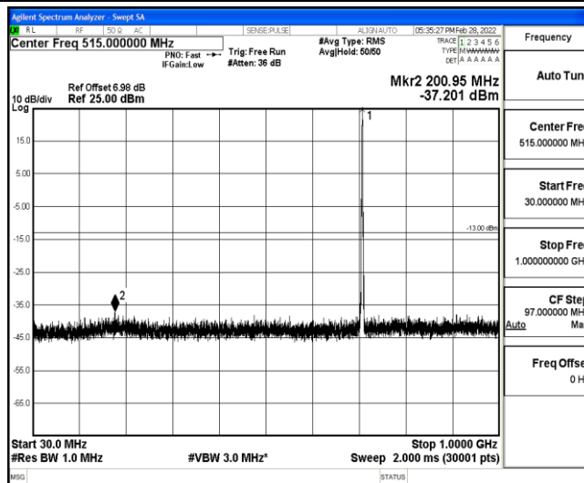
Band12-10MHz-QPSK-23130-1-0-High-30-1000--37.2-PASS
