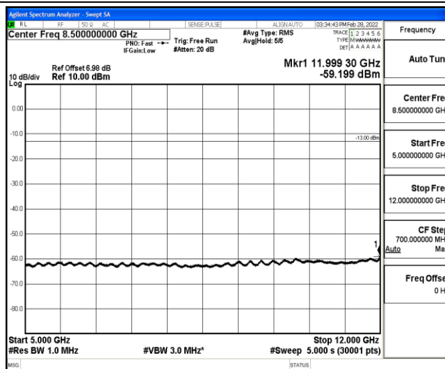
Band12-3MHz-QPSK-23165-1-0-High-5000-12000--59.2-PASS
