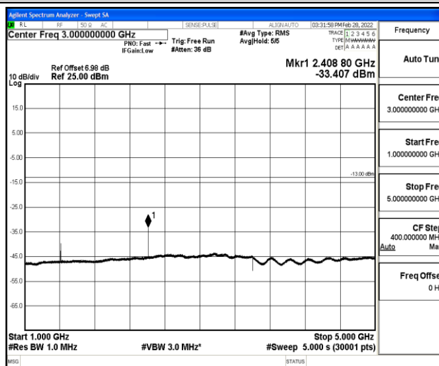
Band12-3MHz-16QAM-23095-1-0-Low-1000-5000--33.41-PASS
