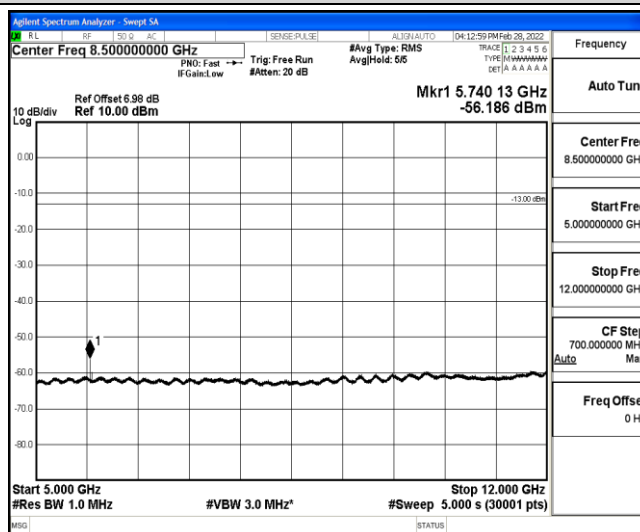
Band12-5MHz-QPSK-23095-1-0-Low-5000-12000--56.19-PASS
