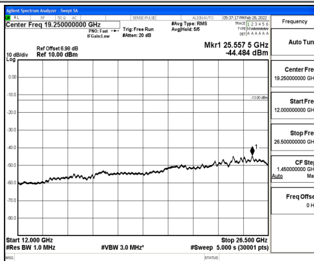
Band12-10MHz-QPSK-23130-1-0-High-12000-26500--44.48-PASS
