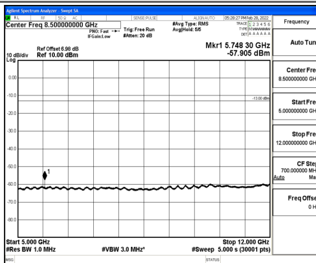
Band12-10MHz-QPSK-23060-1-0-Low-5000-12000--57.91-PASS
