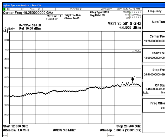
Band12-10MHz-QPSK-23095-1-0-Low-12000-26500--44.51-PASS
