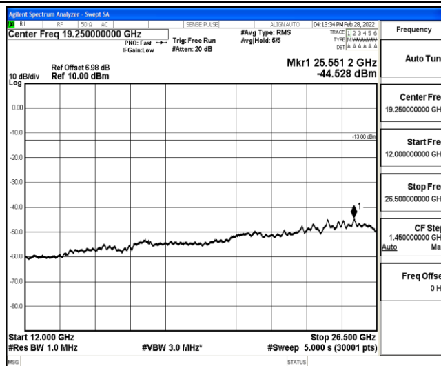
Band12-5MHz-QPSK-23095-1-0-Low-12000-26500--44.53-PASS
