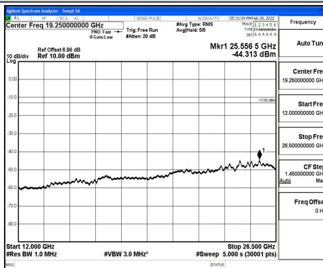
Band12-10MHz-16QAM-23060-1-0-Low-12000-26500--44.31-PASS
