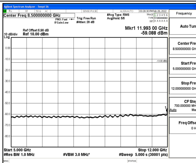
Band12-3MHz-16QAM-23025-1-0-Low-5000-12000--59.09-PASS
