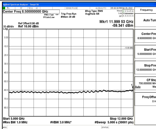
Band12-10MHz-16QAM-23060-1-0-Low-5000-12000--59.34-PASS
