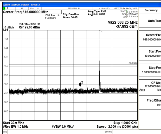
Band12-10MHz-16QAM-23130-1-0-High-30-1000--37.89-PASS
