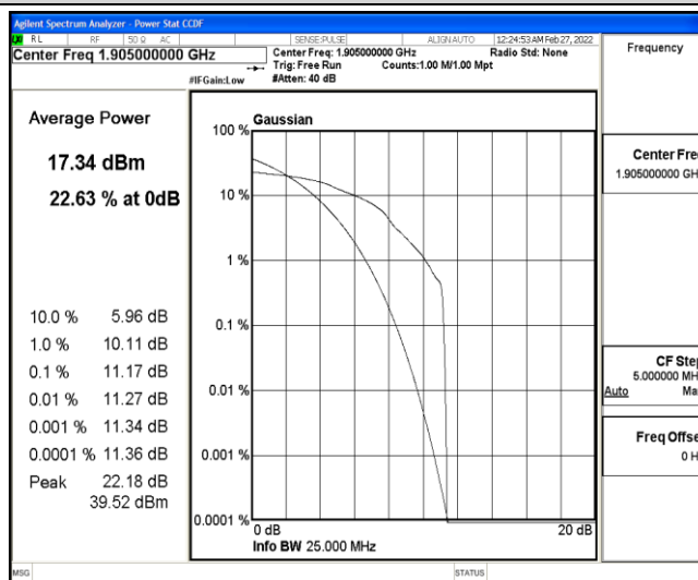
Band25-20MHz-16QAM-26590-1-0-High-11.17-<=13-PASS
