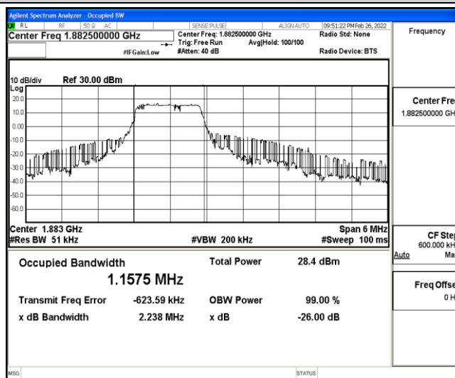
Band25-3MHz-QPSK-26365-6-0-Low-1.1575-2.238-PASS
