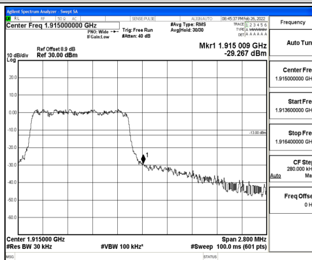
Band25-1.4MHz-16QAM-26683-6-0-High--29.27-PASS
