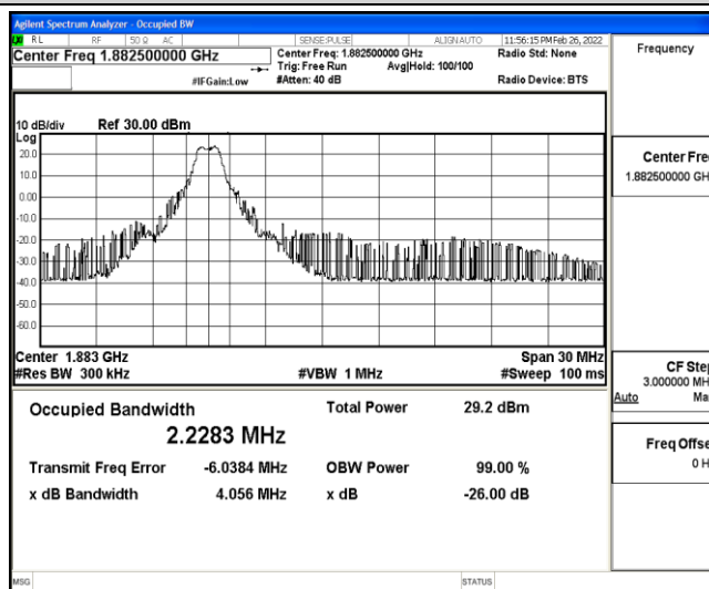
Band25-15MHz-QPSK-26365-6-0-Low-2.2283-4.056-PASS
