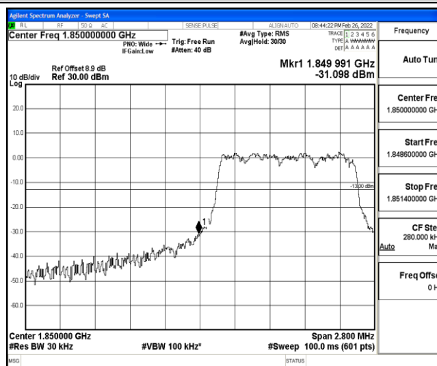
Band25-1.4MHz-QPSK-26047-6-0-Low--31.10-PASS
