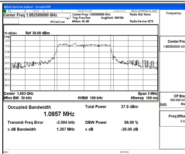
Band25-1.4MHz-16QAM-26365-6-0-Low-1.0857-1.267-PASS
