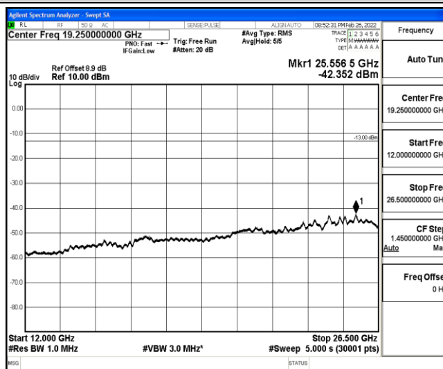
Band25-1.4MHz-16QAM-26047-1-0-Low-12000-26500--42.35-PASS
