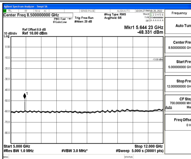
Band25-3MHz-16QAM-26365-1-0-Low-5000-12000--48.33-PASS
