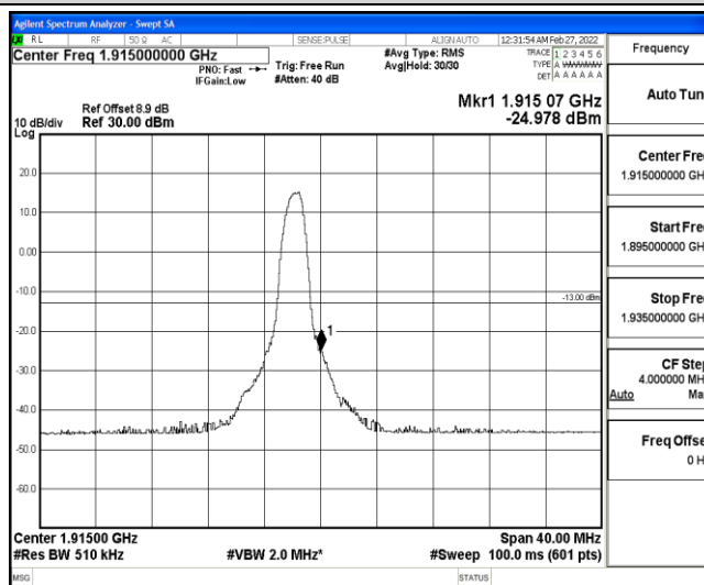
Band25-20MHz-QPSK-26590-6-0-High--24.98-PASS
