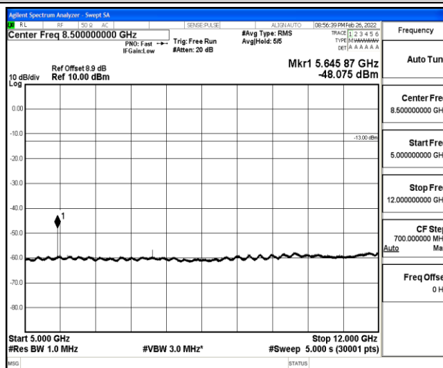
Band25-1.4MHz-QPSK-26365-1-0-Low-5000-12000--48.08-PASS
