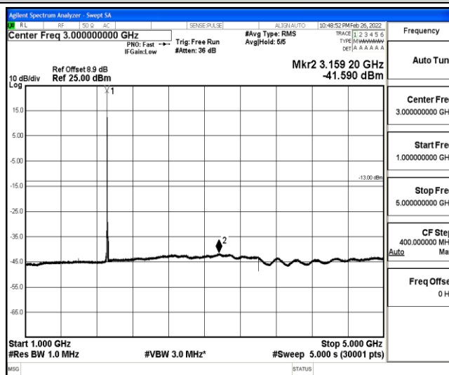
Band25-5MHz-16QAM-26665-1-0-High-1000-5000--41.59-PASS
