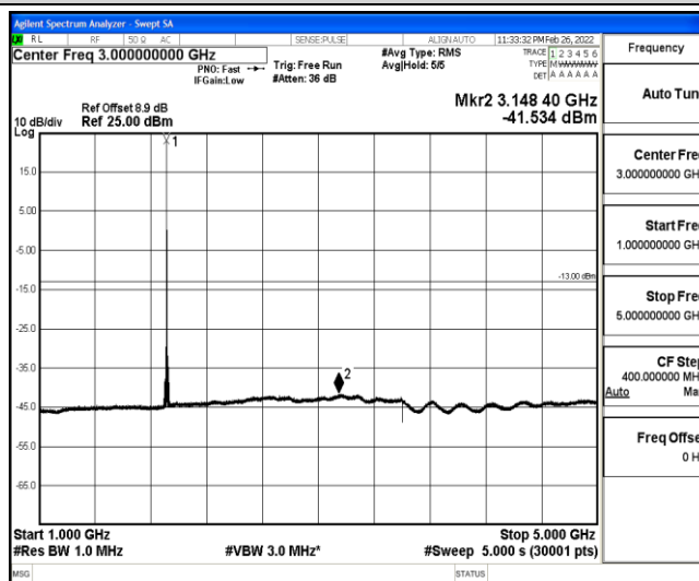
Band25-10MHz-QPSK-26640-1-0-High-1000-5000--41.53-PASS
