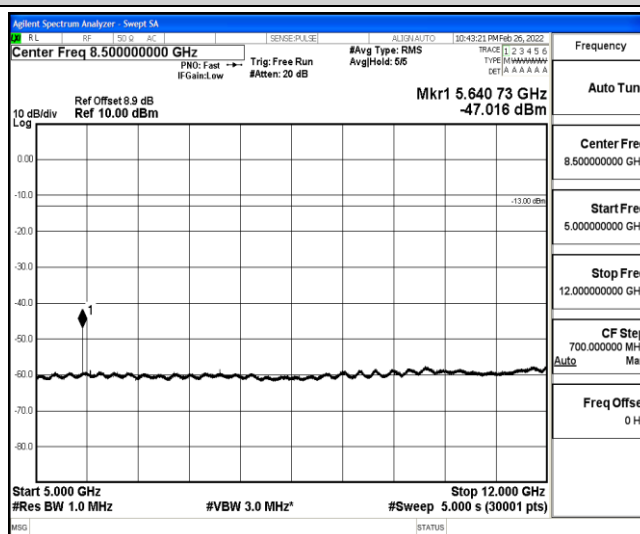
Band25-5MHz-QPSK-26365-1-0-Low-5000-12000--47.02-PASS
