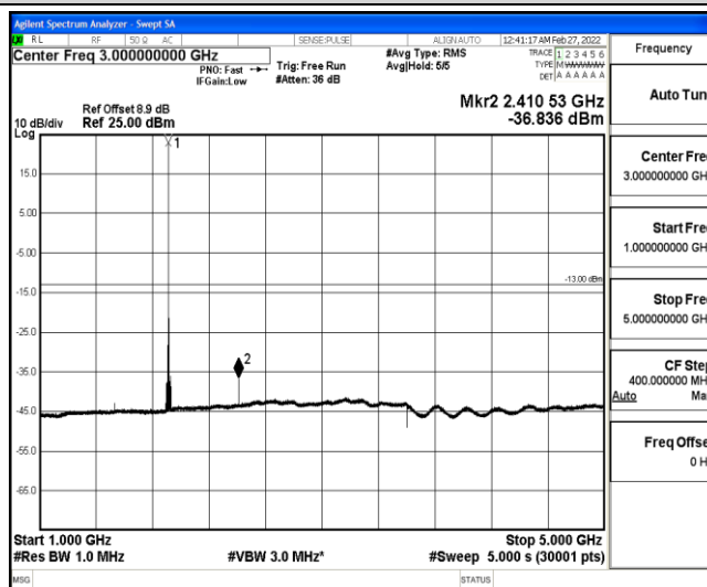
Band25-20MHz-QPSK-26590-1-0-High-1000-5000--36.84-PASS
