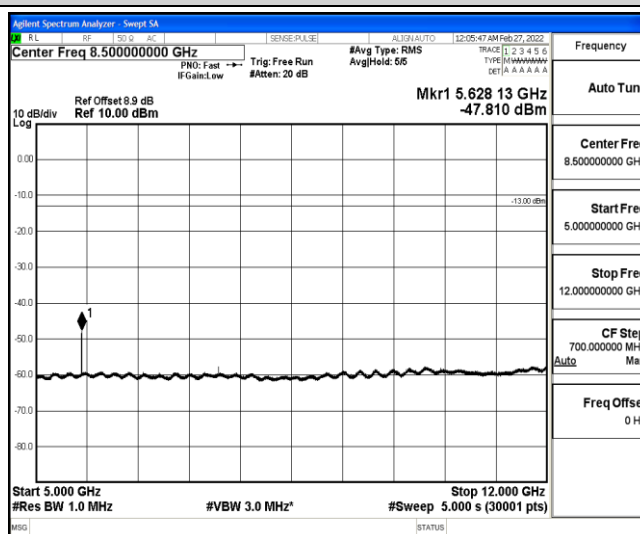
Band25-15MHz-QPSK-26365-1-0-Low-5000-12000--47.81-PASS
