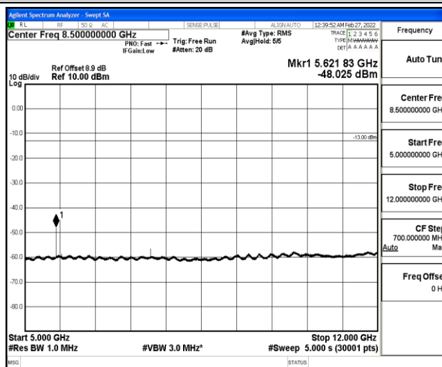
Band25-20MHz-16QAM-26365-1-0-Low-5000-12000--48.03-PASS
