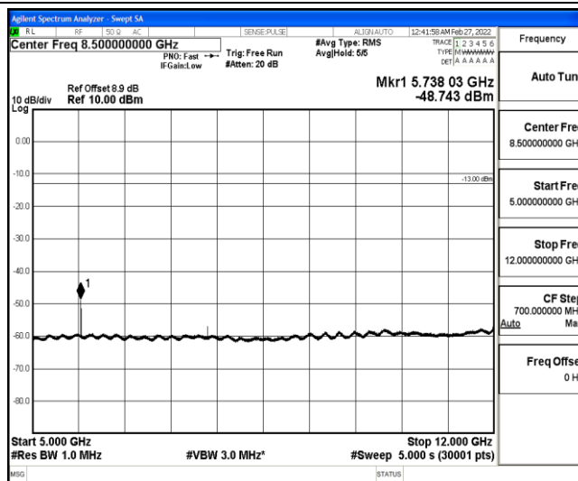
Band25-20MHz-QPSK-26590-1-0-High-5000-12000--48.74-PASS
