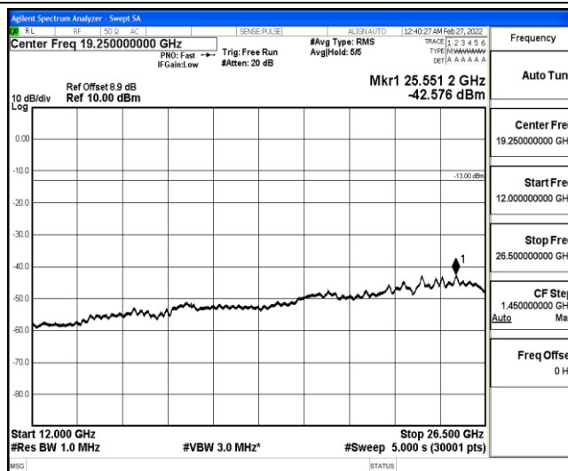
Band25-20MHz-16QAM-26365-1-0-Low-12000-26500--42.58-PASS
