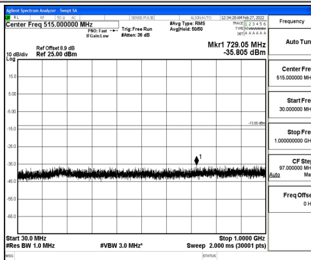
Band25-20MHz-16QAM-26140-1-0-Low-30-1000--35.81-PASS
