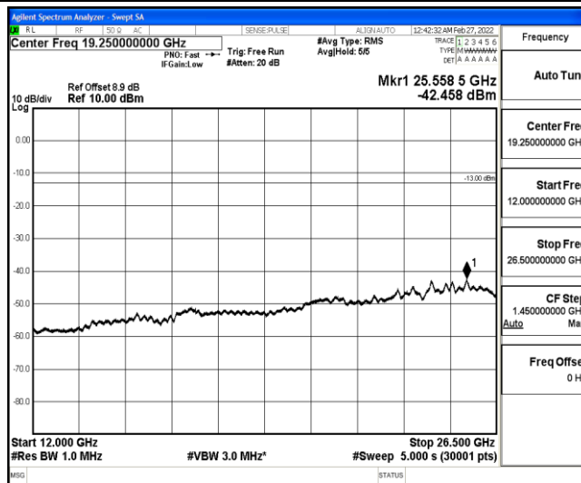
Band25-20MHz-QPSK-26590-1-0-High-12000-26500--42.46-PASS
