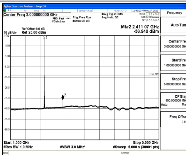
Band25-20MHz-16QAM-26590-1-0-High-1000-5000--36.94-PASS
