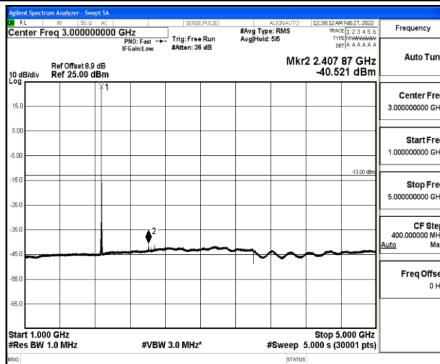
Band25-20MHz-16QAM-26365-1-0-Low-1000-5000--40.52-PASS
