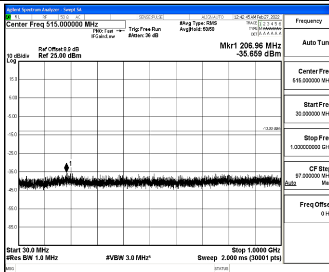
Band25-20MHz-16QAM-26590-1-0-High-30-1000--35.66-PASS
