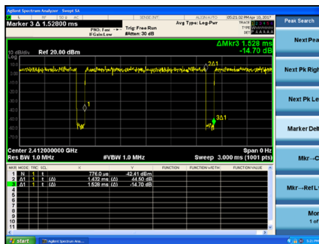
Duty Cycle_802.11g
