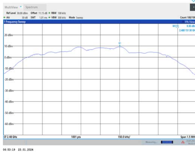
3DH5 Ant1_2480
