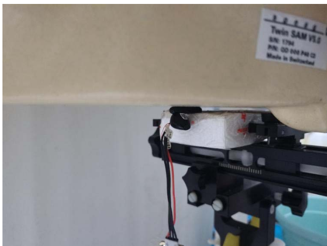
Fig-4.1 Rear Side of EUT with 0 cm Gap (Head Mode)
