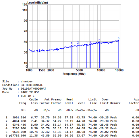
BLE_1M_TX_CH_00_Horizontal-Peak
