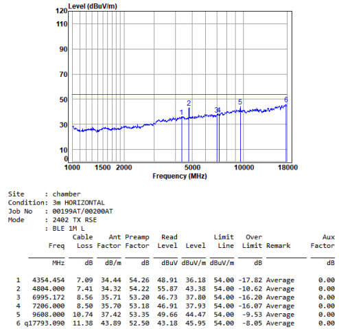
BLE_1M_TX_CH_00_Horizontal-Avg
