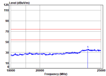
Left BT_TX_CH_M_Vertical
