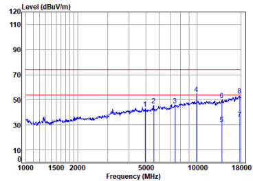
Right BT_DH5_TX_CH_78_Vertical
