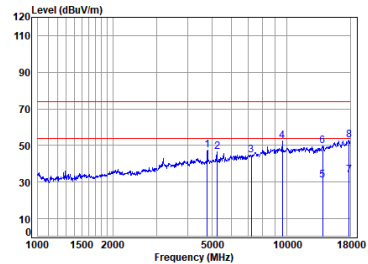
Left BT_DH5_TX_CH_00_Vertical
