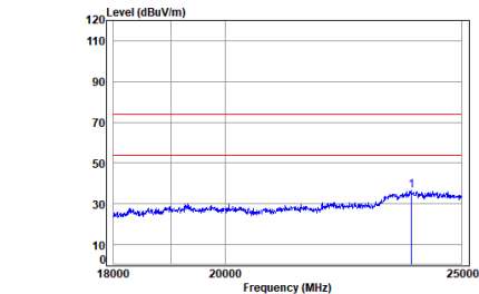
Right BT_TX_CH_M_Horizontal
