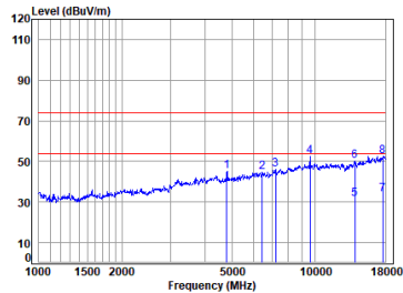
Right BT_DH5_TX_CH_00_Horizontal
