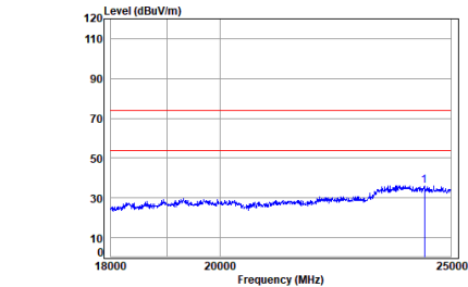
Left BT_TX_CH_M_Horizontal
