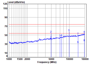
Left BT_DH5_TX_CH_78_Vertical
