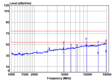
Left BT_DH5_TX_CH_39_Vertical
