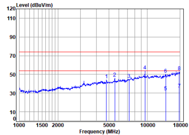
Right BT_DH5_TX_CH_00_Vertical
