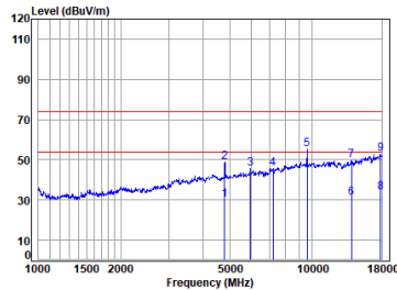
Left BT_DH5_TX_CH_00_Horizontal
