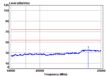
Right BT_TX_CH_M_Vertical
