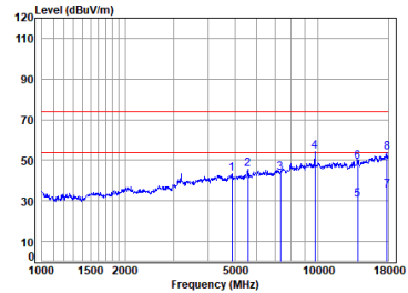
Right BT_DH5_TX_CH_39_Vertical
