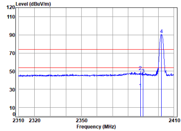
Left BT_DH5_TX_CH_00_Vertical
