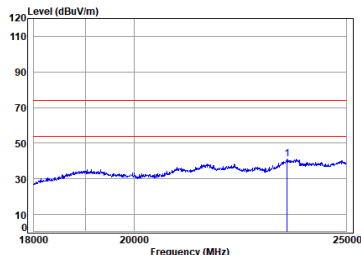
BT_DH5_TX_CH_78_Vertical
