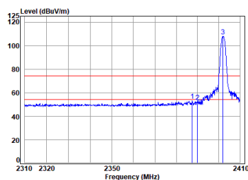
BT_DH5_TX_CH_00_Vertical
