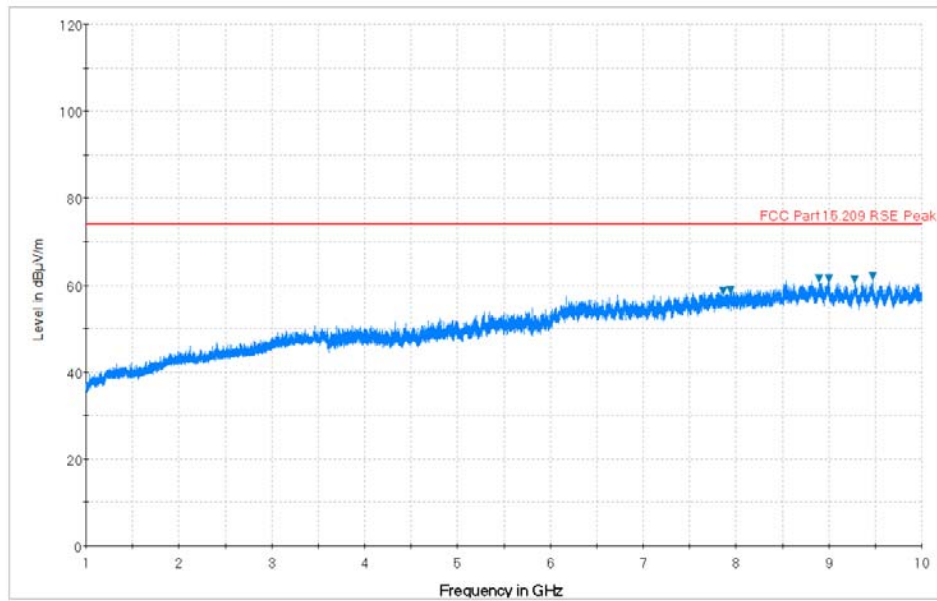
Plot 7-23. Radiated Spurious Plot above 1GHz (High Channel, Ant. Pol. V)
