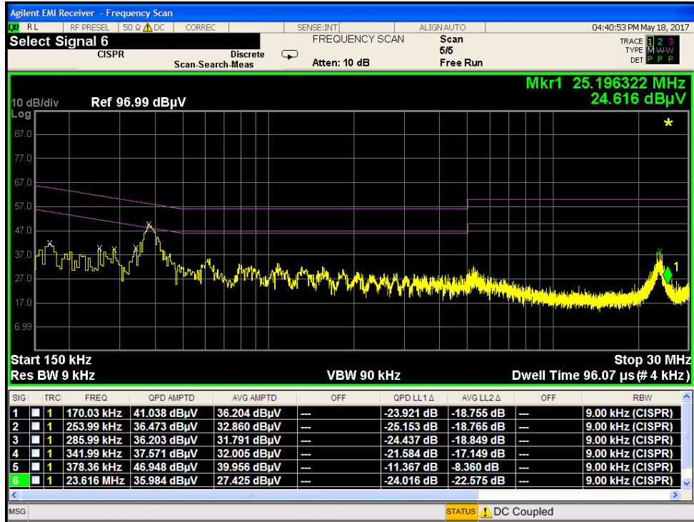
Plot 7-26. Line Conducted Plot (L1)
