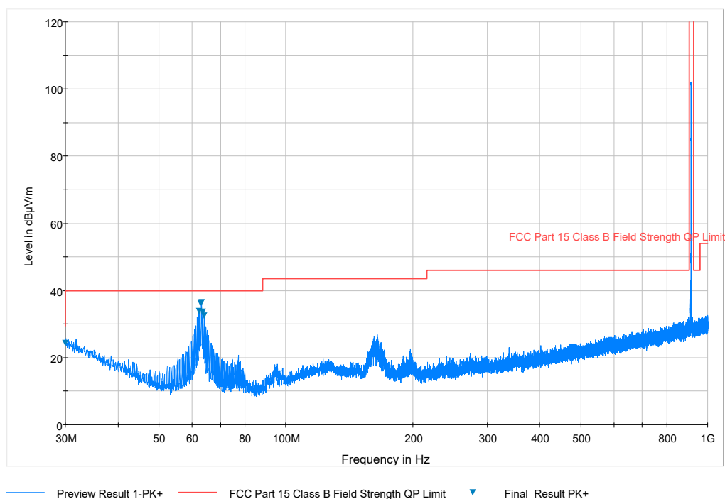
Plot 7-24. Radiated Spurious Plot below 1GHz (Pol. H)
