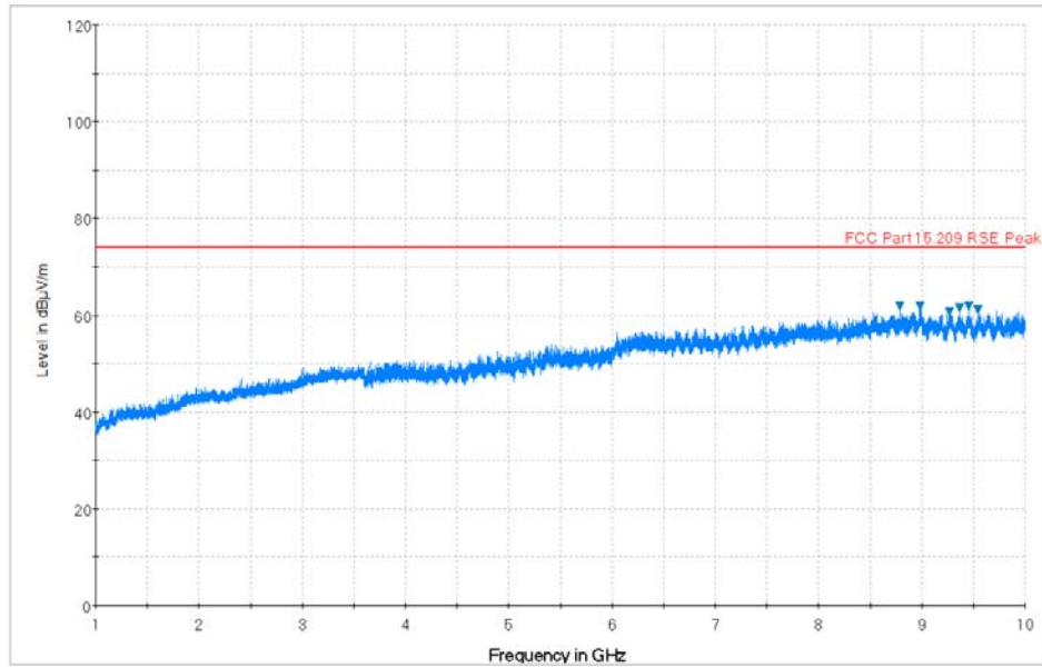
Plot 7-21. Radiated Spurious Plot above 1GHz (Mid Channel, Ant. Pol. V)
