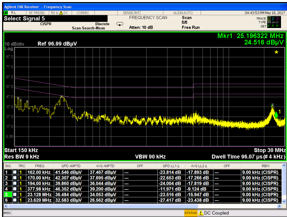
Plot 7-27. Line Conducted Plot (N)
