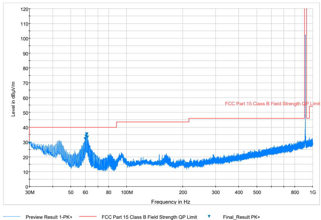
Plot 7-25. Radiated Spurious Plot below 1GHz (Pol. V)
