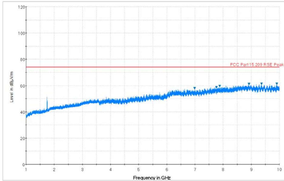
Plot 7-20. Radiated Spurious Plot above 1GHz (Mid Channel, Ant. Pol. H)
