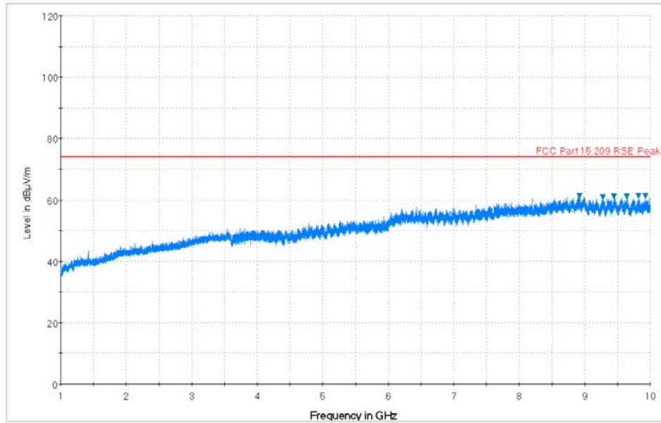
Plot 7-22. Radiated Spurious Plot above 1GHz (High Channel, Ant. Pol. H)
