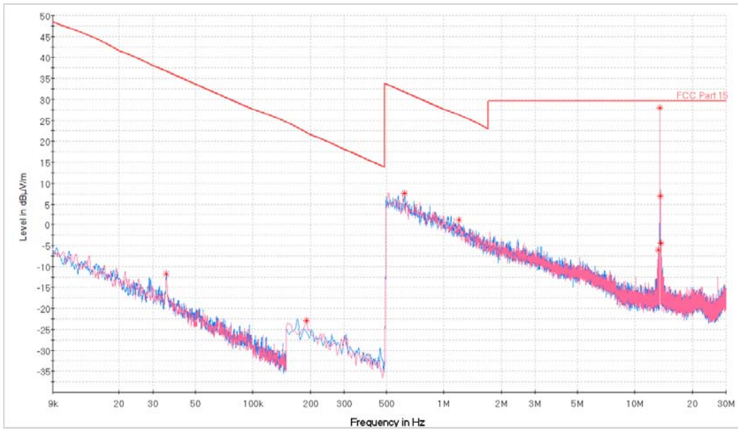
Plot 7-11. Radiated Spurious Plot 9kHz – 30MHz (Pol. X)
