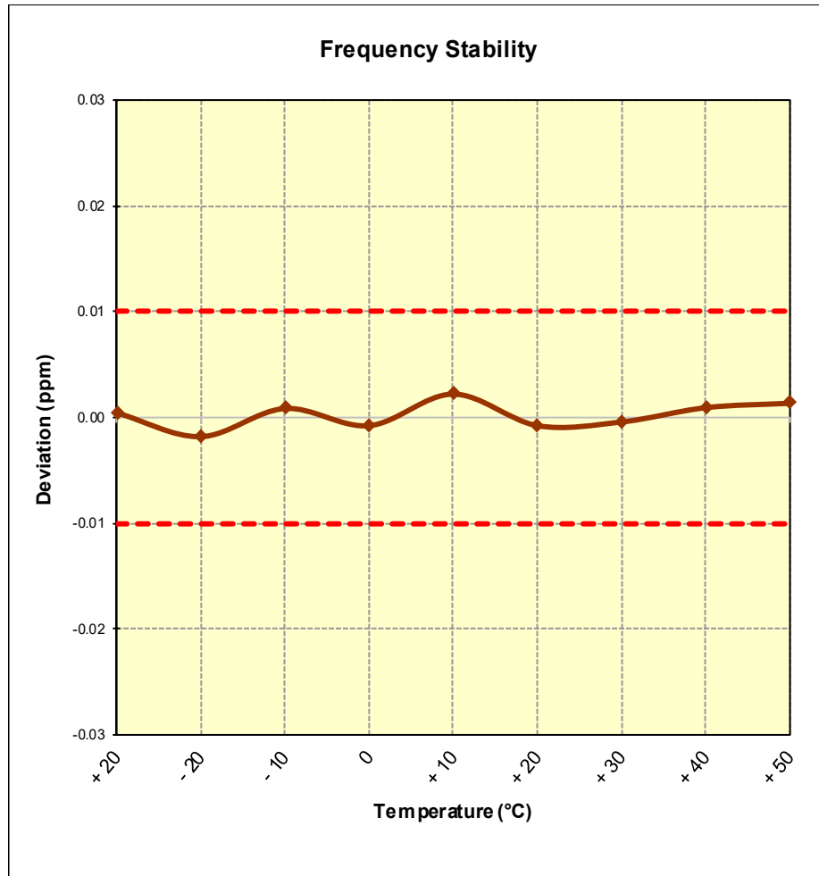
Figure 7-5. Frequency Stability Plot
