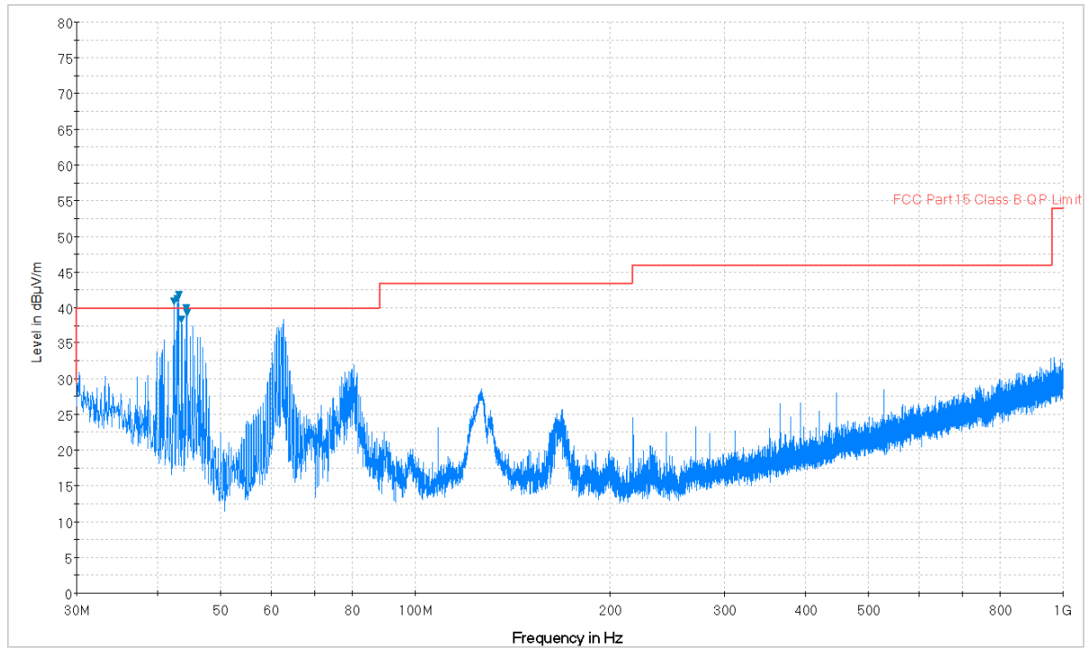
Plot 7-5. Radiated Spurious Plot 30MHz – 1GHz (Pol. V)
