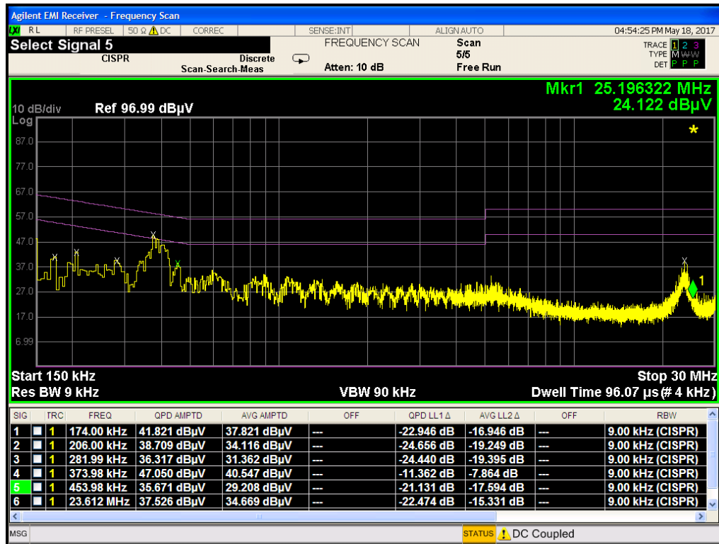
Plot 7-18. Line-Conducted Test Plot (L1, RFID Antenna Terminated in 50Ω) (160143-915 (H318))
