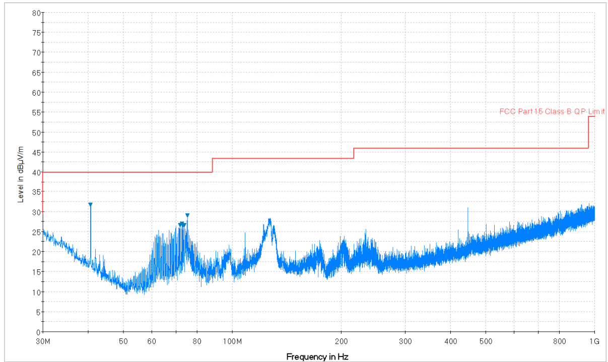
Plot 7-9. Radiated Spurious Plot 30MHz – 1GHz (Pol. H)
