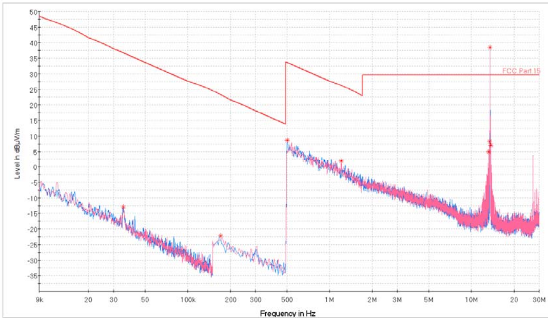
Plot 7-12. Radiated Spurious Plot 9kHz – 30MHz (Pol. Y)
