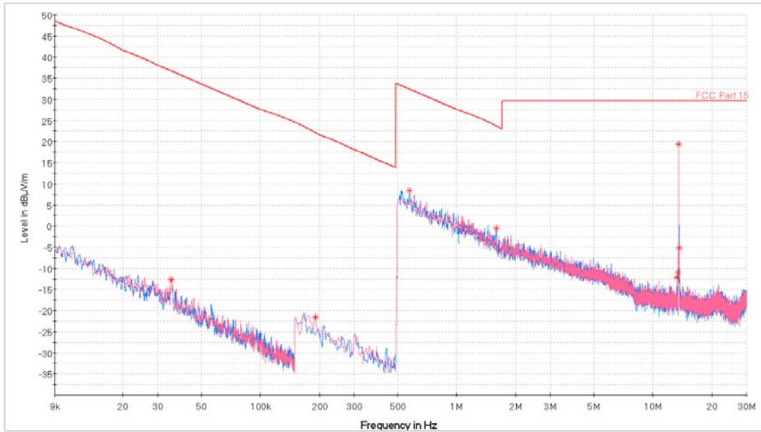
Plot 7-3. Radiated Spurious Plot 9kHz – 30MHz (Pol. Z)
