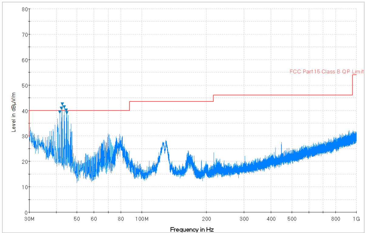
Plot 7-15. Radiated Spurious Plot 30MHz – 1GHz (Pol. V)
