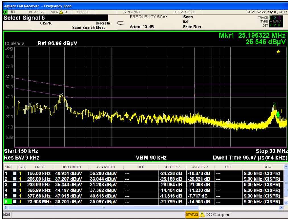
Plot 7-20. Line-Conducted Test Plot (L1, RFID Antenna Terminated in 50Ω) (160132-915 (R318))
