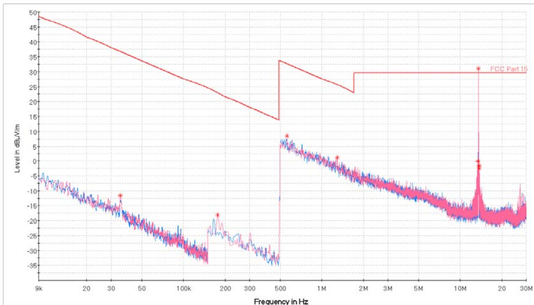
Plot 7-2. Radiated Spurious Plot 9kHz – 30MHz (Pol. Y)
