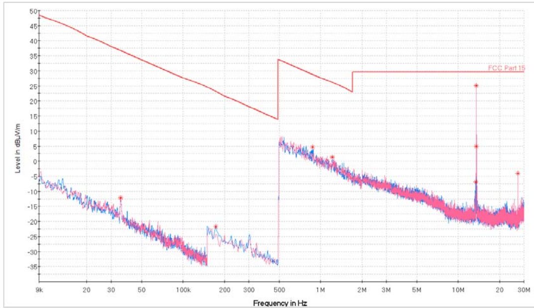
Plot 7-8. Radiated Spurious Plot 9kHz – 30MHz (Pol. Z)
