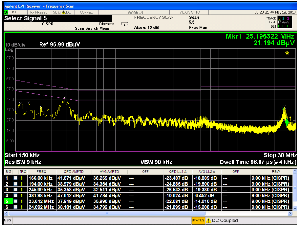
Plot 7-16. Line-Conducted Test Plot (L1, RFID Antenna Terminated in 50Ω) (160117-915 (H218))
