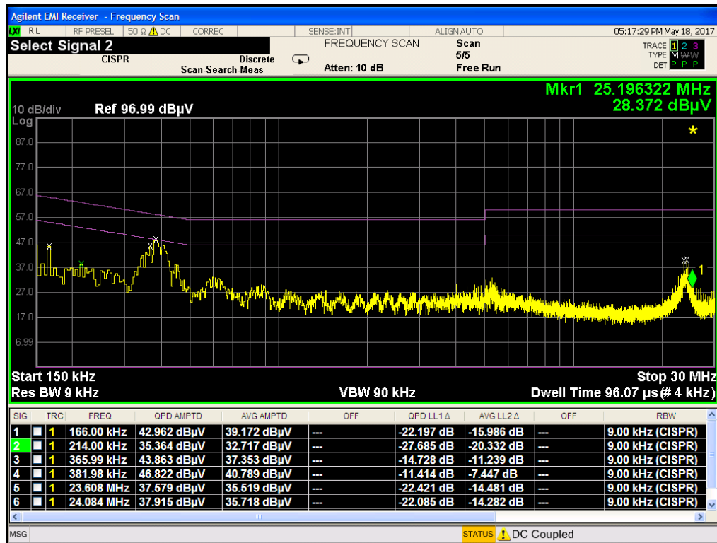
Plot 7-17. Line-Conducted Test Plot (N, RFID Antenna Terminated in 50Ω) (160117-915 (H218))
