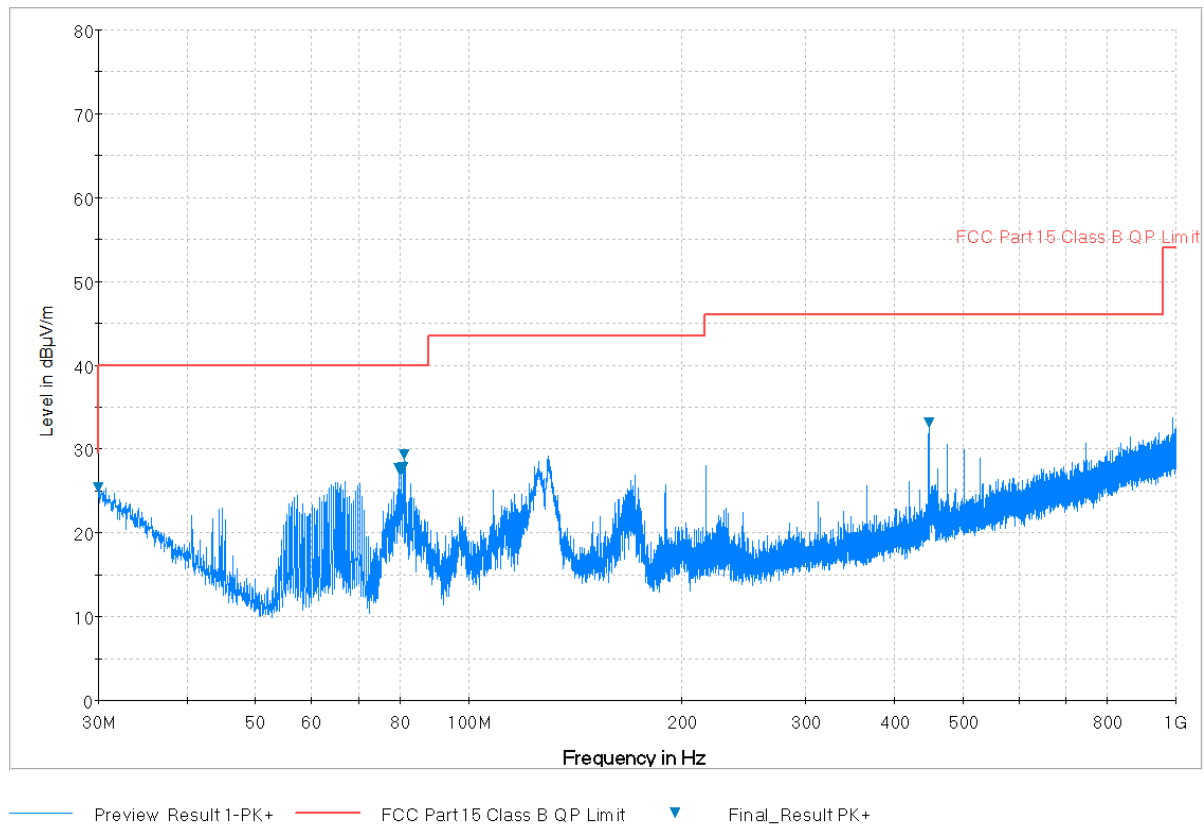
Plot 7-14. Radiated Spurious Plot 30MHz – 1GHz (Pol. H)
