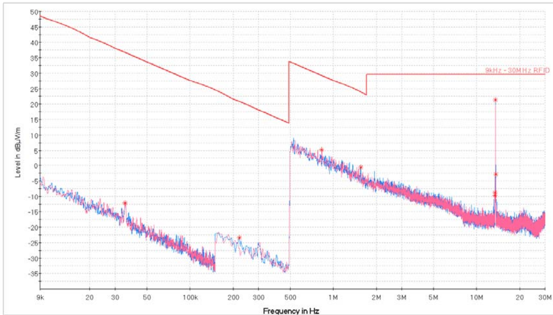
Plot 7-1. Radiated Spurious Plot 9kHz – 30MHz (Pol. X)
