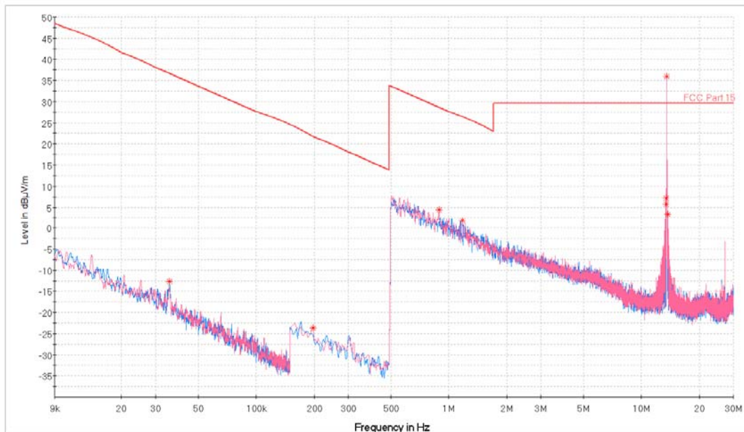
Plot 7-7. Radiated Spurious Plot 9kHz – 30MHz (Pol. Y)
