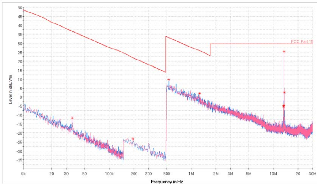
Plot 7-6. Radiated Spurious Plot 9kHz – 30MHz (Pol. X)
