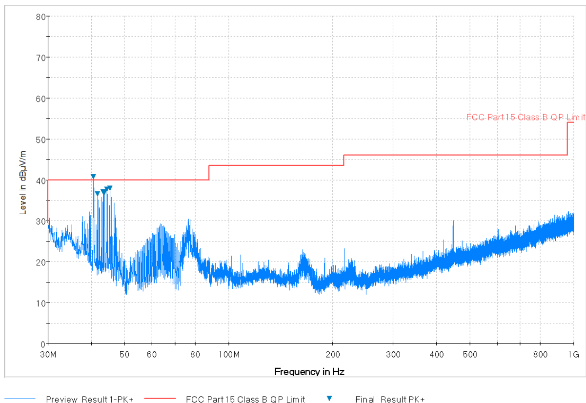
Plot 7-10. Radiated Spurious Plot 30MHz – 1GHz (Pol. V)
