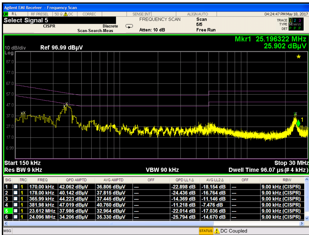
Plot 7-21. Line-Conducted Test Plot (N, RFID Antenna Terminated in 50Ω) (160132-915 (R318))
