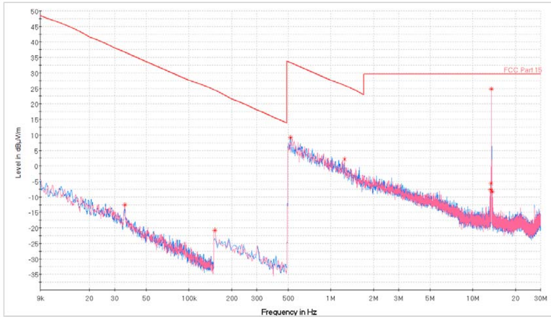
Plot 7-13. Radiated Spurious Plot 9kHz – 30MHz (Pol. Z)
