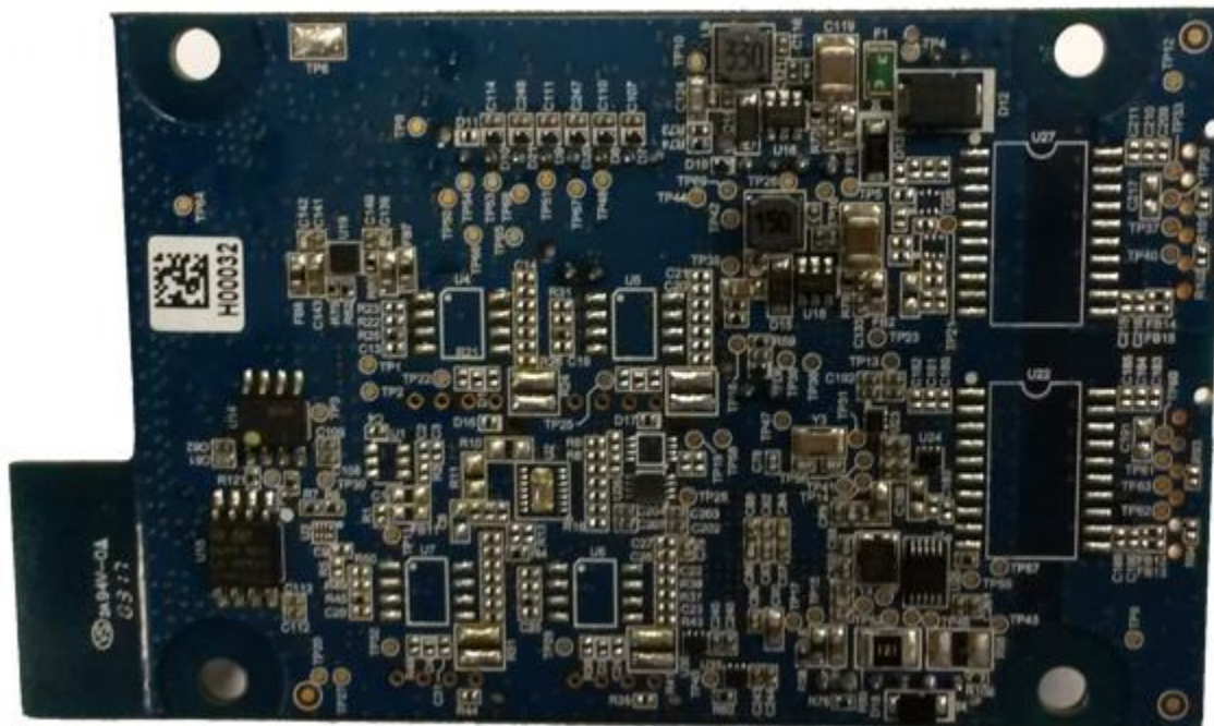
Sensor PCB – Bottom:
