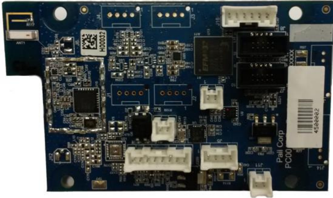
Sensor PCB – Top:
