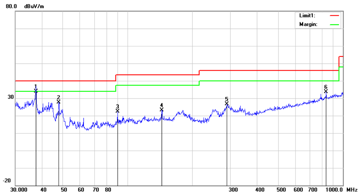
Vertical Polarity Plot @3m
