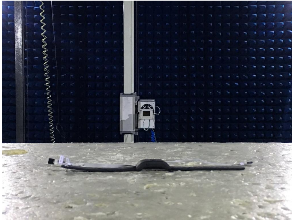
Photograph 5: Set-up for Spurious Emissions (18GHz-26GHz)
