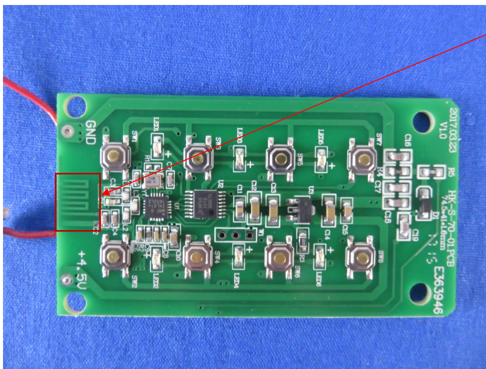
2434MHz Antenna
