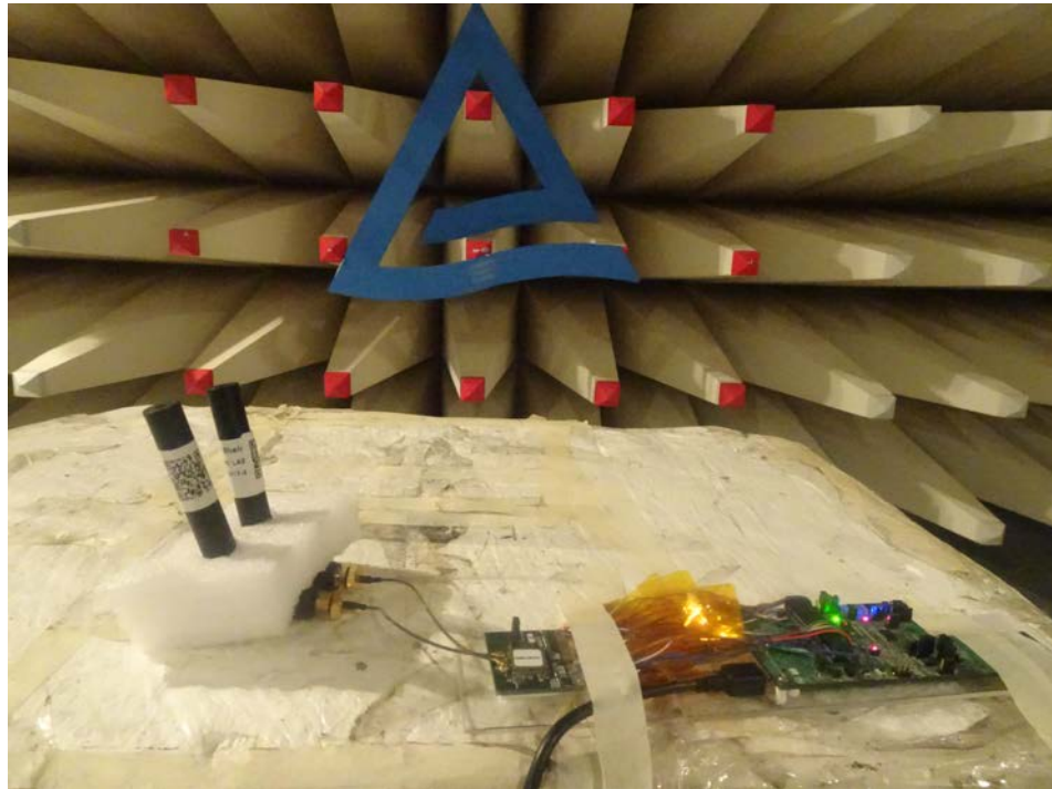
Test Setup
