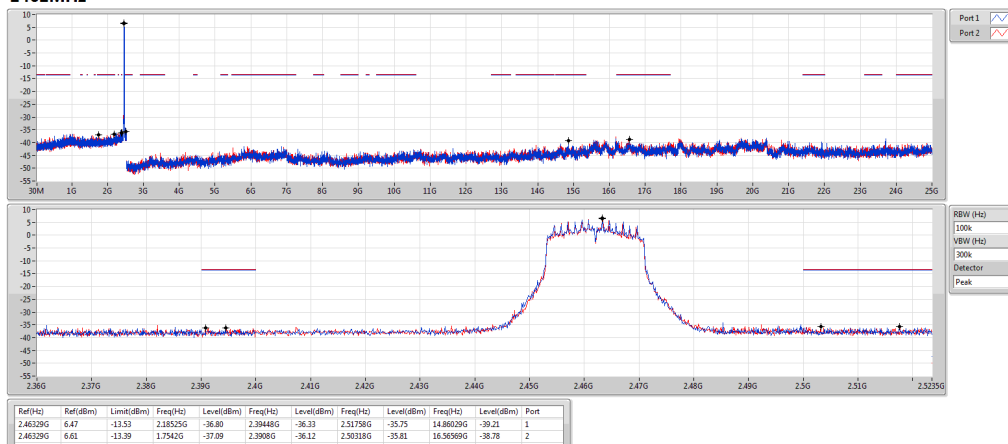
802.11n HT20_Nss1,(MCS0)_2TX
