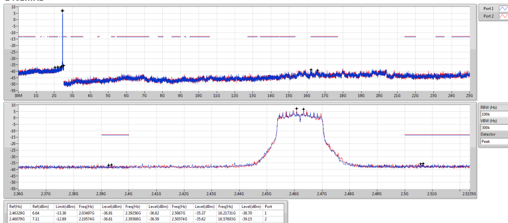
802.11g_Nss1,(6Mbps)_2TX
