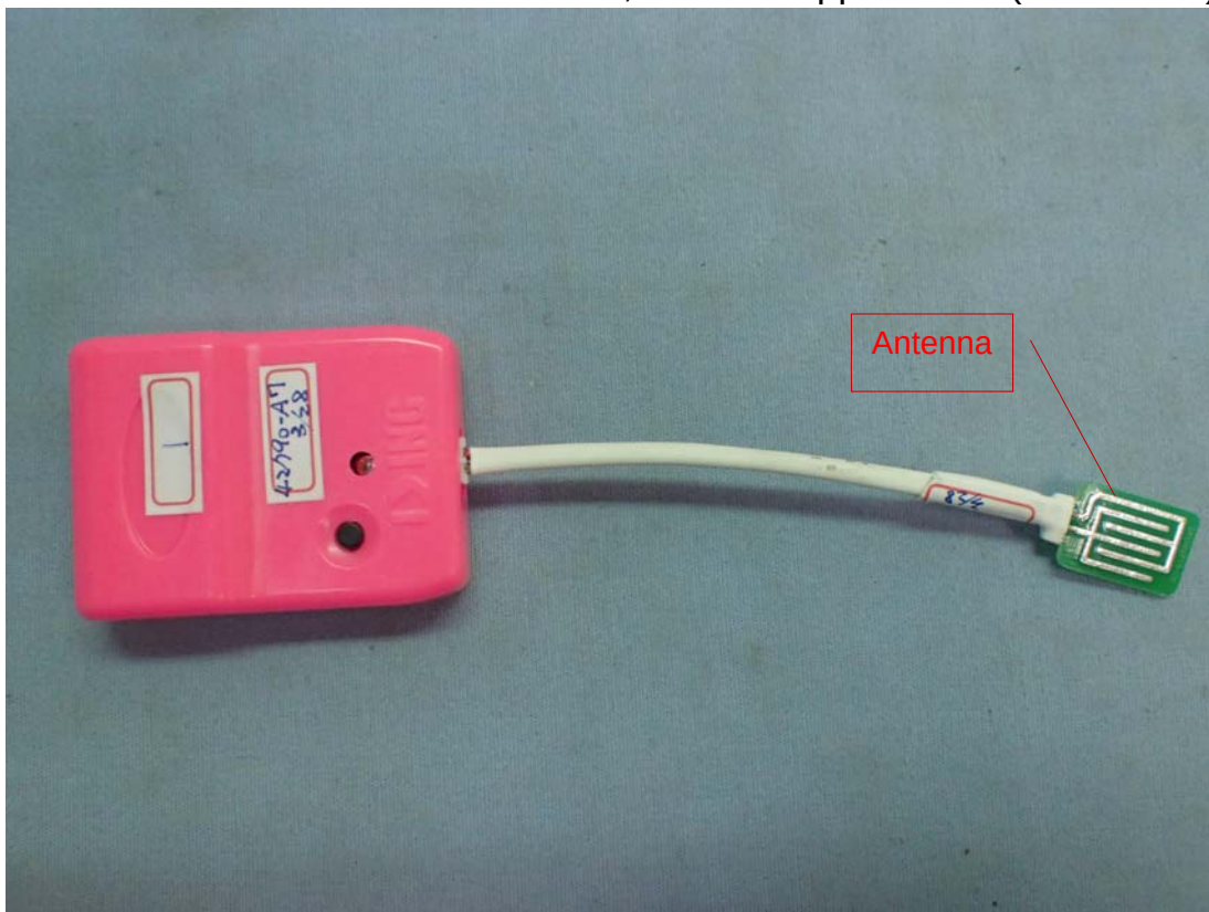
Figure 1 Transmitter+Sensor, General Appearance (Front View)
