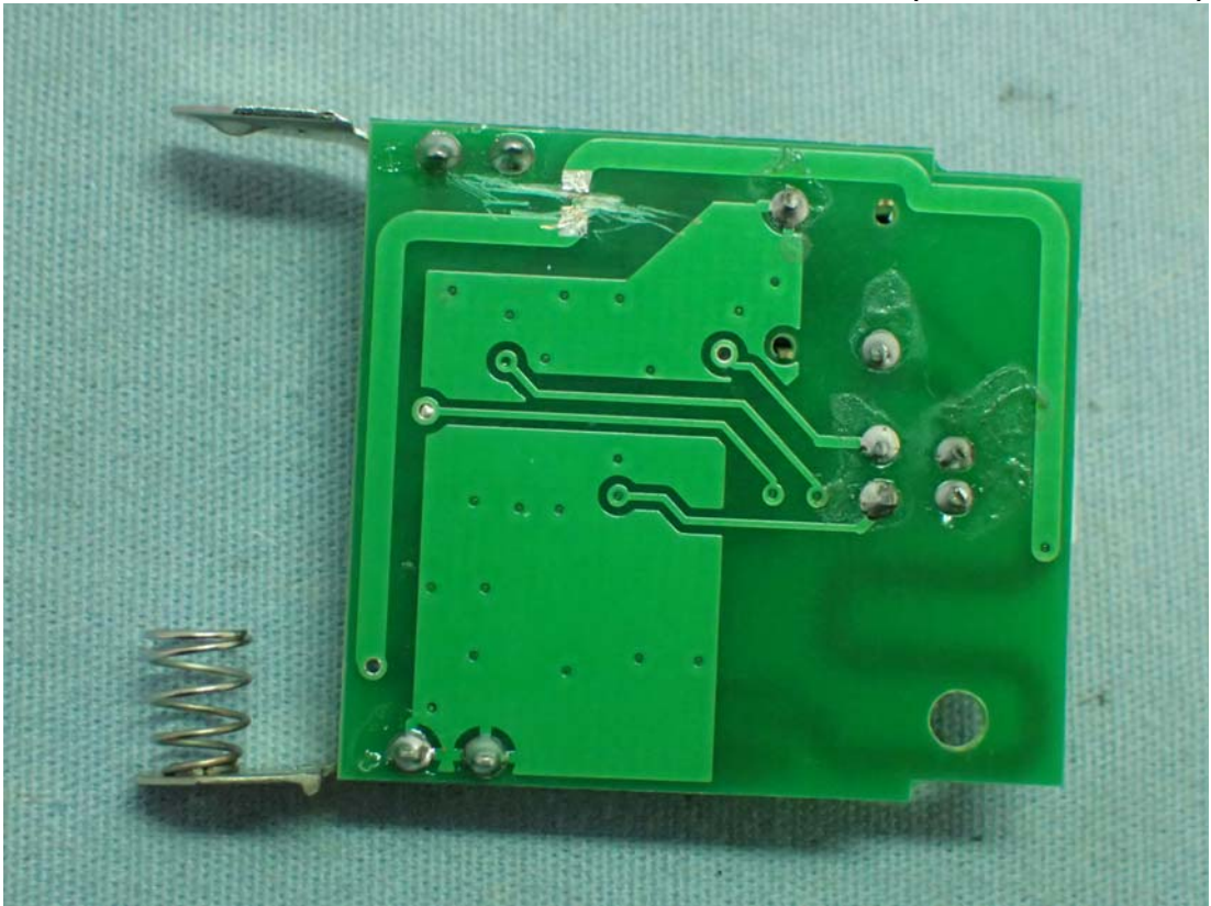
Figure 10 Alarm, Internal View (PCB, Back View)
