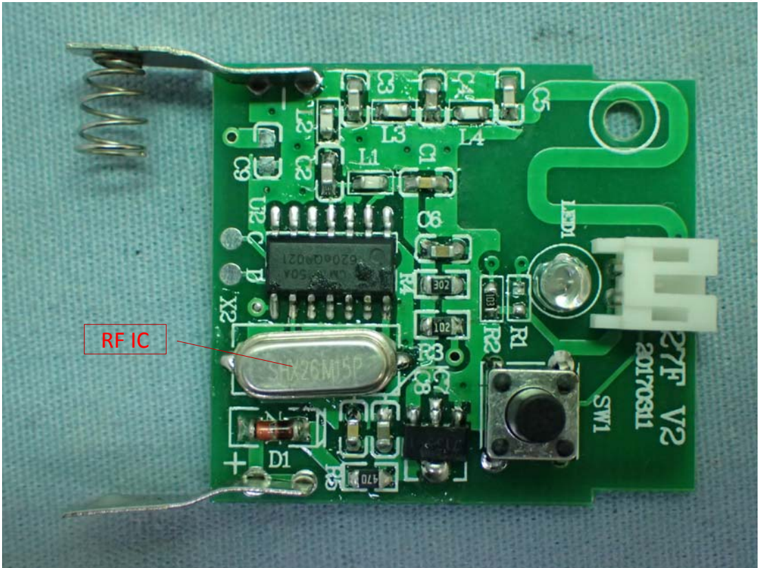
Figure 9 Alarm, Internal View (PCB, Front View)
