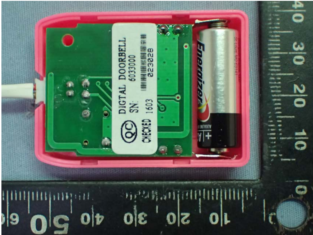
Figure 7 Transmitter, Internal View
