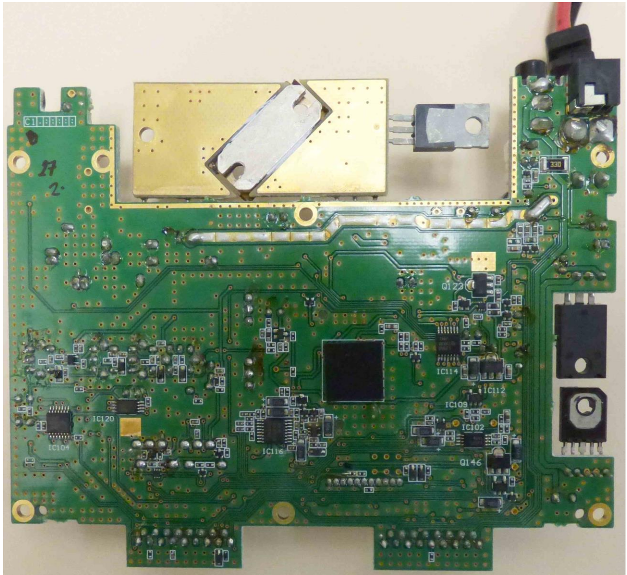
Main logic board – Rear side
