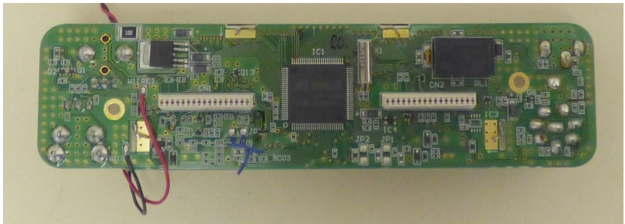
Control head board – Rear side
