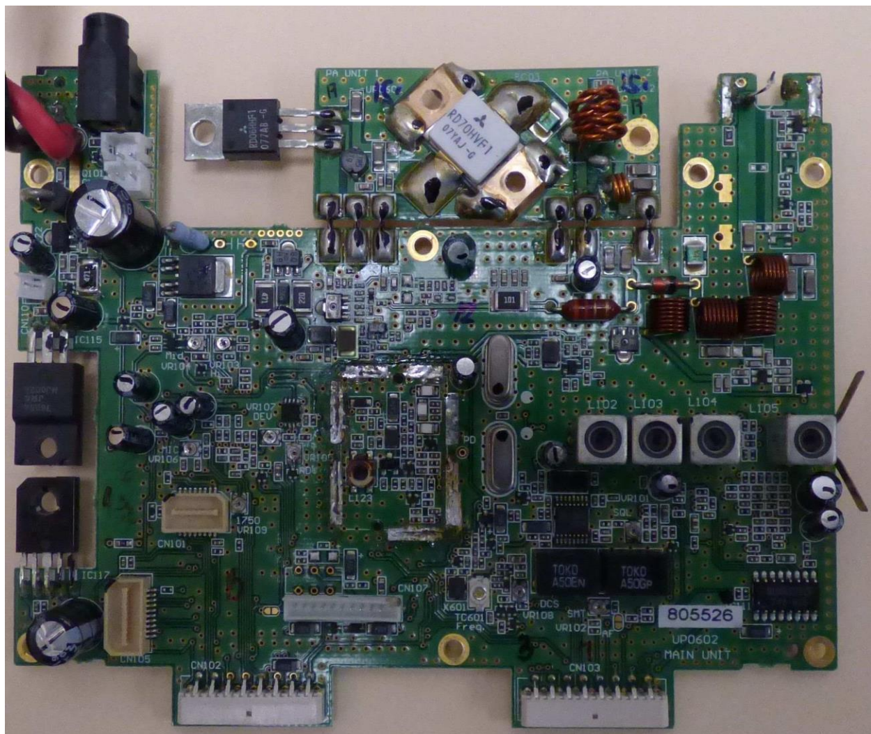
Main logic board – Without RF shield
