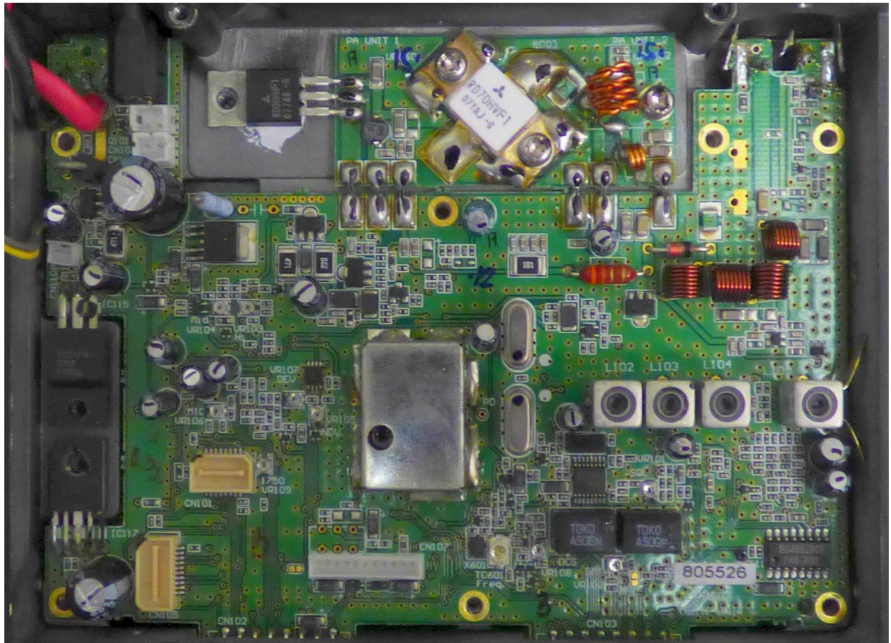
Main logic board – With RF shield
