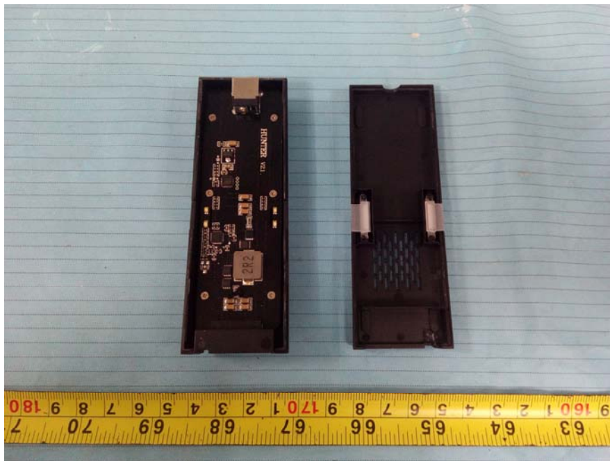
EUT – Cover off View 1 (Battery Charger)
