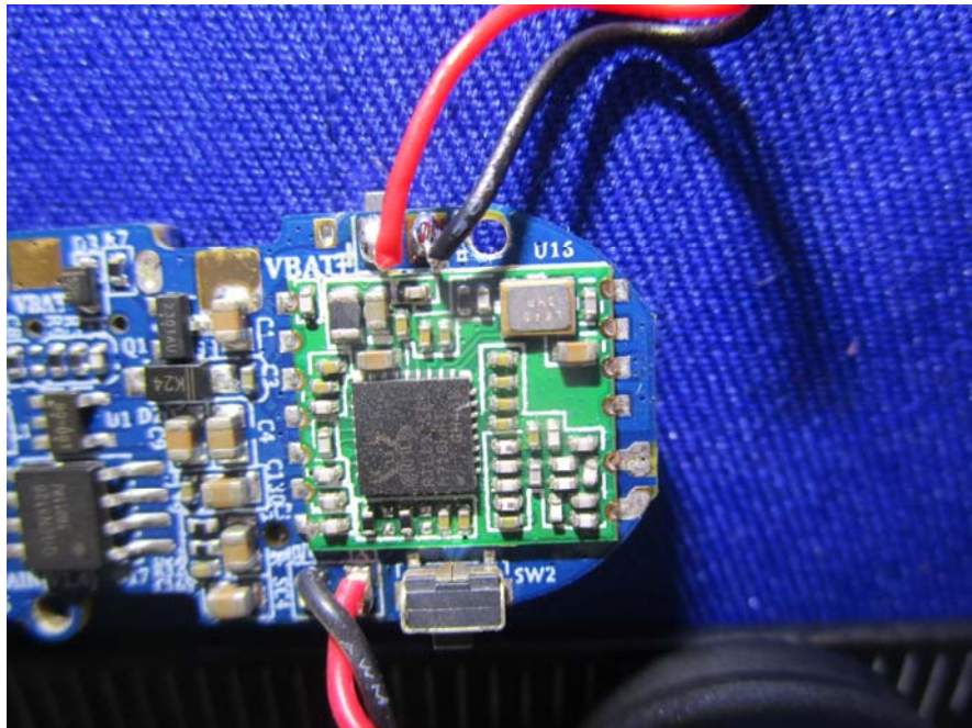
EUT –Wifi PCB View
