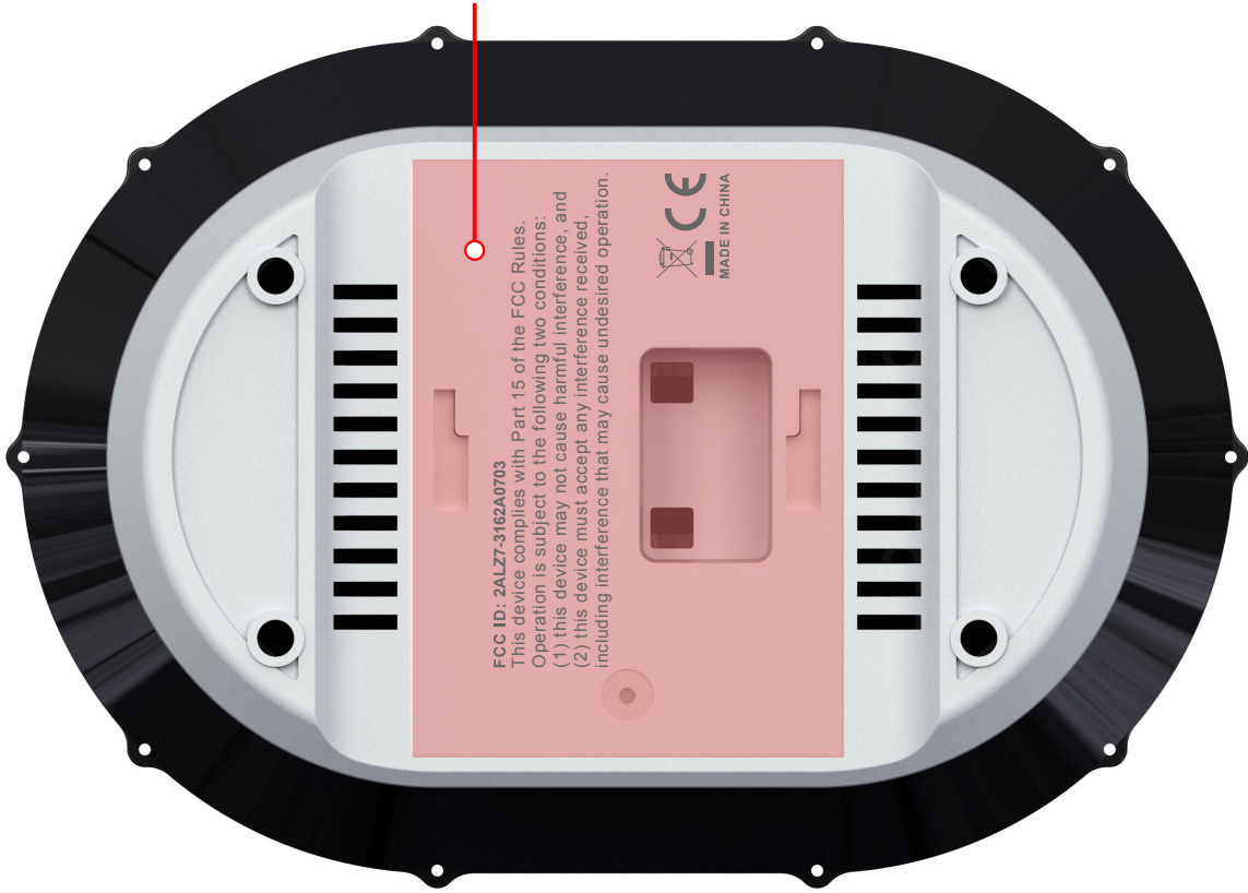
INJECT COL: #331626(GRAY) StURFACE TREATMENT: GW-1128(Fine Matte Surface) RED ZONE POLISHING WORD & SYMBOL: UV LASER ENGRAVING
