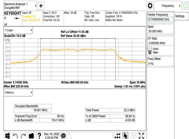
802.11a_20MHz_Chain0_5745MHz
