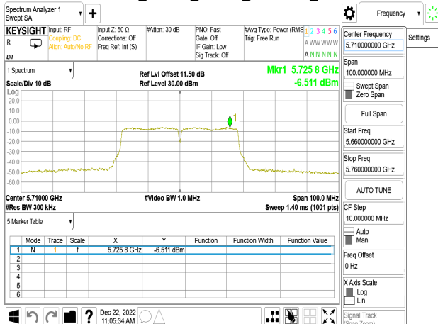
802.11n_40MHz_Chain0_5710MHz_UNII 3
