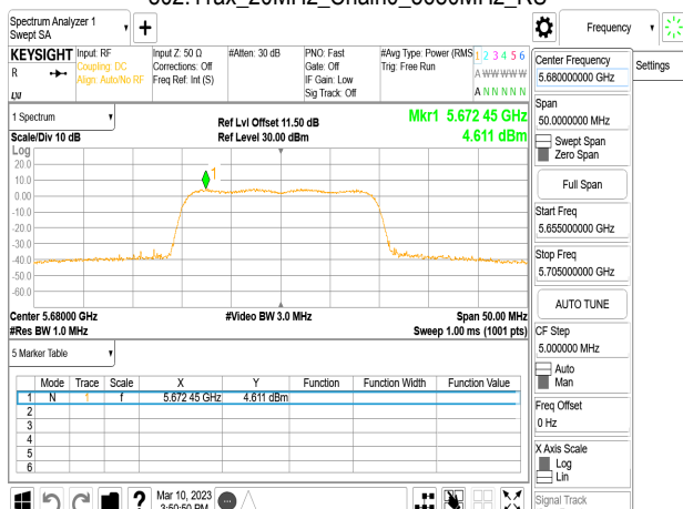
802.11ax_20MHz_Chain0_5680MHz_RU106_53
