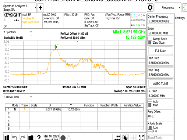
802.11ax_20MHz_Chain0_5680MHz_RU26_8
