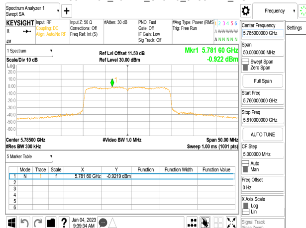
802.11ax_20MHz_Chain0_5785MHz_RU106_53
