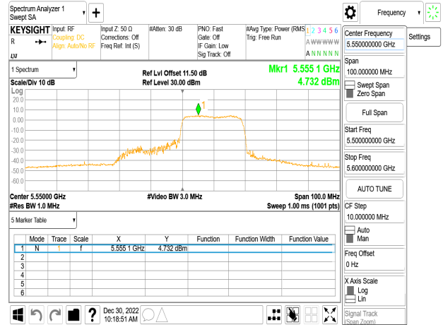
802.11ax_40MHz_Chain0_5550MHz_SU
