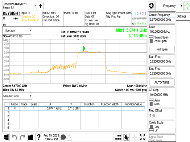
802.11ax_40MHz_Chain0_5670MHz_SU
