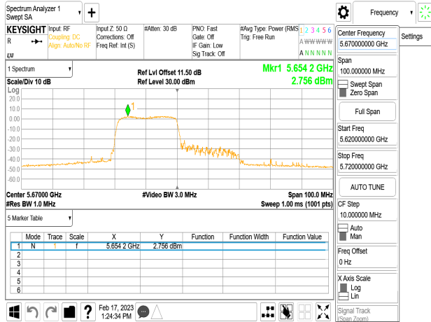
802.11ax_40MHz_Chain0_5670MHz_RU242_62
