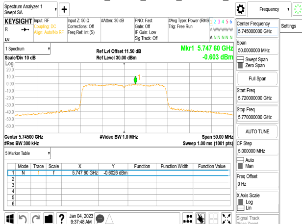
802.11ax_20MHz_Chain0_5745MHz_RU
