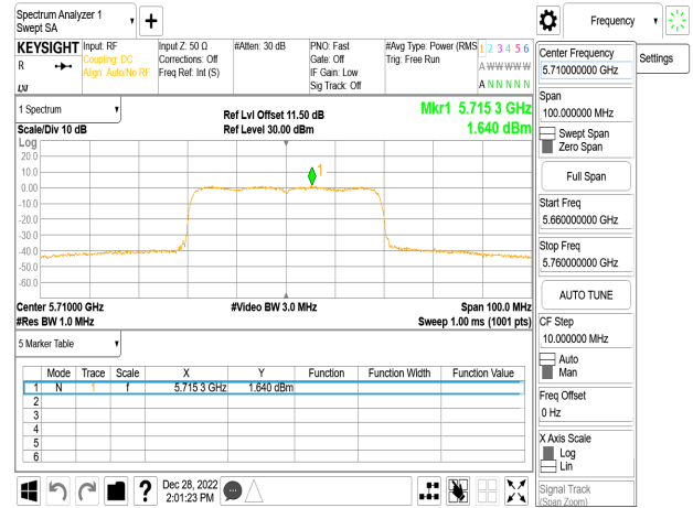
802.11ax_40MHz_Chain0_5710MHz_UNII 3_RU
