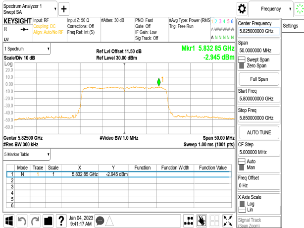
802.11ax_20MHz_Chain0_5825MHz_RU106_53
