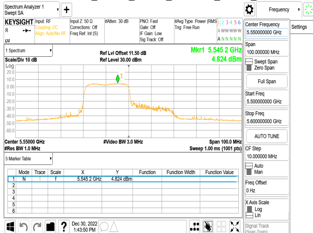
802.11ax_40MHz_Chain0_5550MHz_RU242_61
