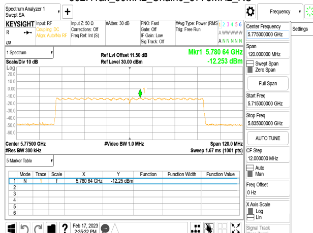
802.11ax_80MHz_Chain0_5775MHz_RU
