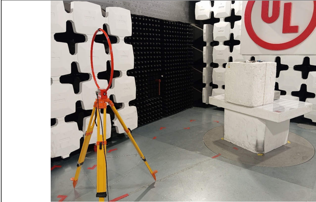
Radiated emission, below 30 MHz (axis X)
