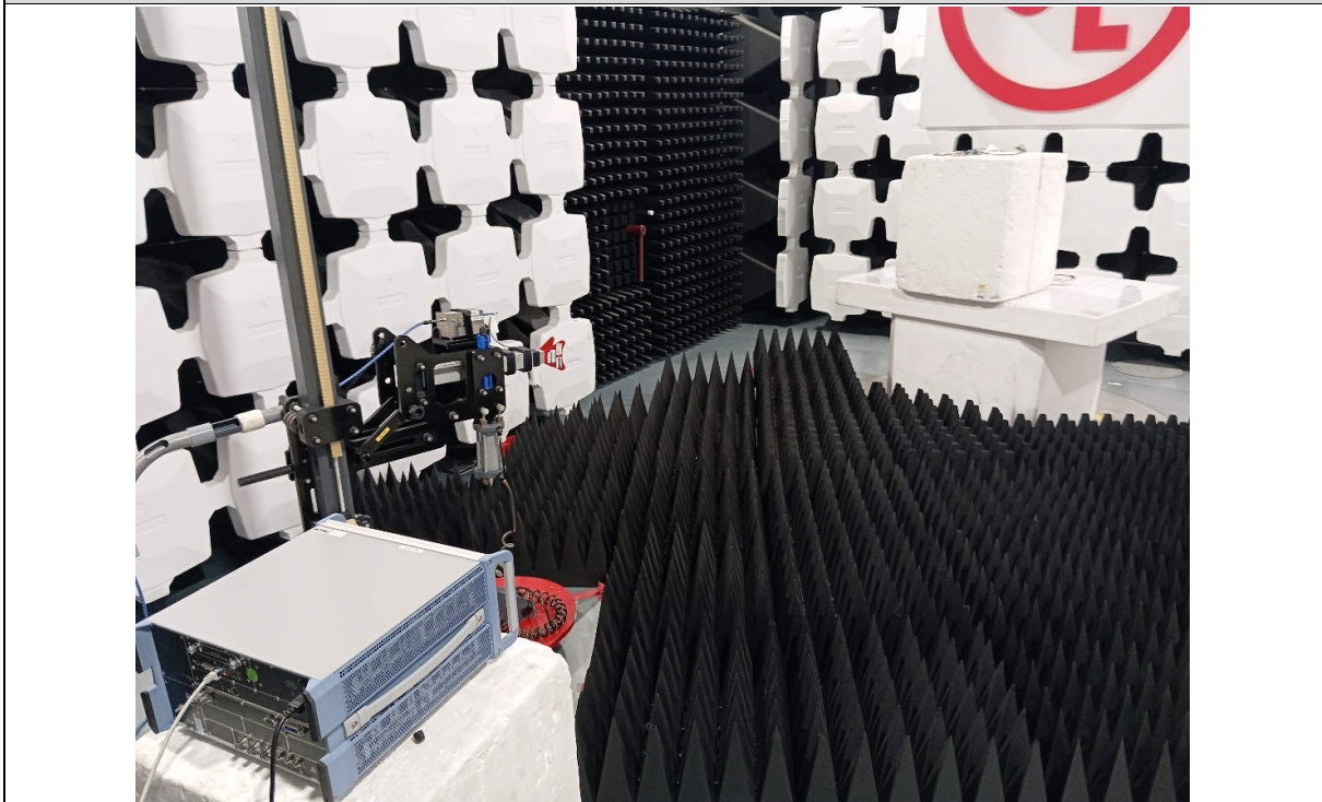
Radiated emission, above 1 GHz
