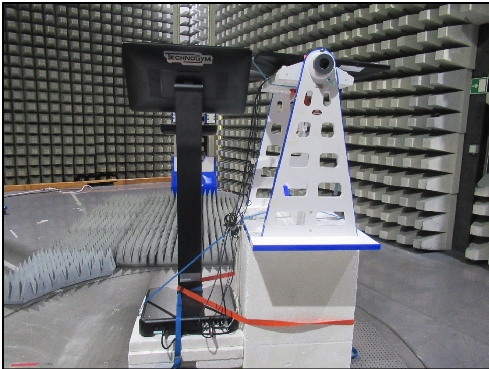
Photo 7 Radiated Test Setup from 1 GHz to 18 GHz
