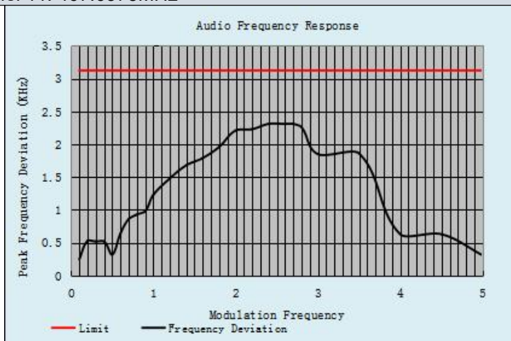
Channel 11: 467.6375MHz
