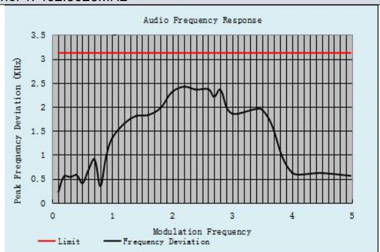
Channel 1: 462.5625MHz
