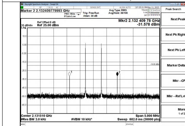
AWS Band Pre AGC, DL
