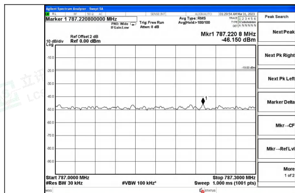
Upper 700MHz band CDMA UL Right Side Pre AGC
