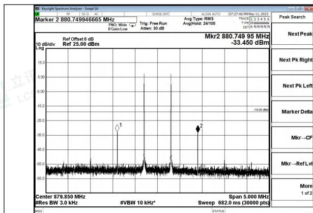
Cellular Band Pre AGC, DL
