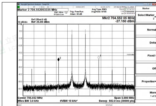
Lower 700MHz band Pre AGC, UL
