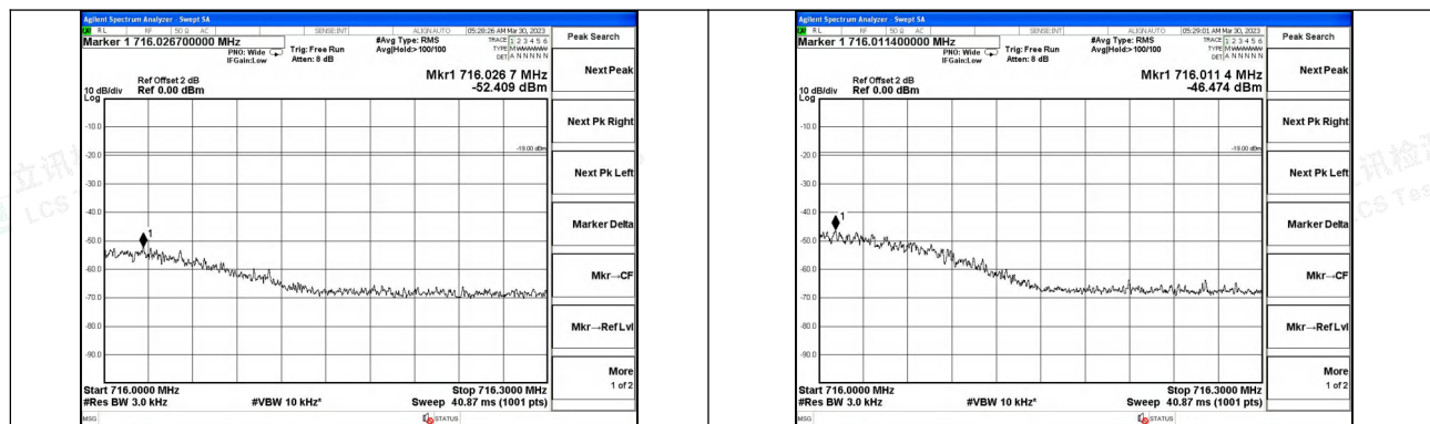
Lower 700MHz band GSM UL Right Side Pre AGC
