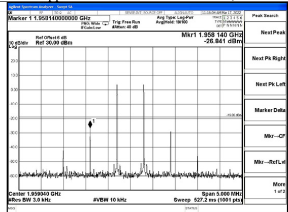
PCS Band AGC+10dB, DL
