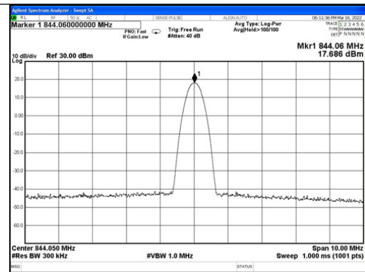
Cellular Band CW, UL
