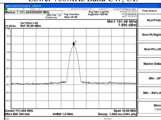
Lower 700MHz Band CW, DL
