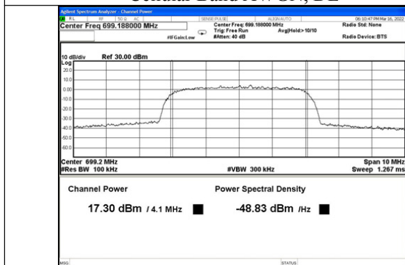
Lower 700MHz Band AWGN, UL
