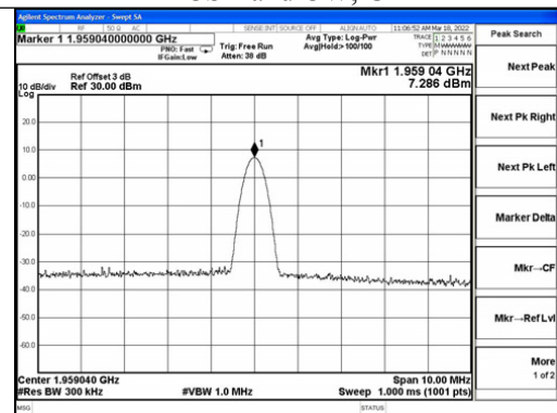
PCS Band CW, DL
