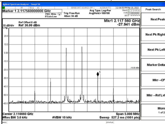
AWS Band Pre AGC, DL
