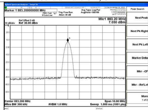
Cellular Band CW, DL
