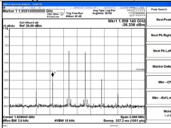
PCS Band Pre AGC, DL
