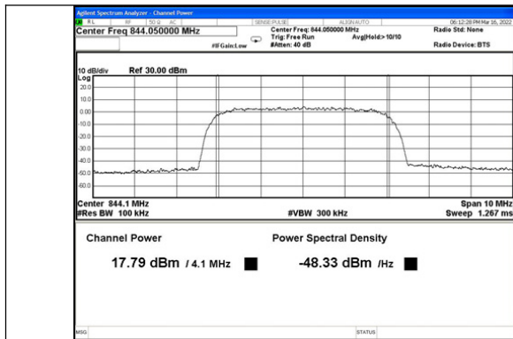
Cellular Band AWGN, UL
