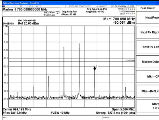
Lower 700MHz band Pre AGC, UL
